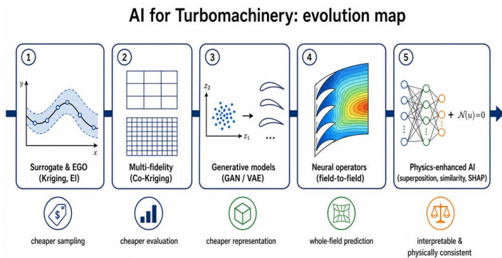
AI4Turbomachinery evolution map (English labels; this lecture is stage 3: generative model)
