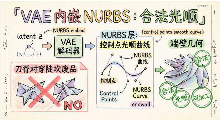
NURBS embed VAE: 解码器内嵌光顺层过合法三关
