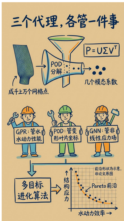
POD 压缩与 GPR/POD/GNN 三代理分工 (pod three surrogates, 手绘手账版)
