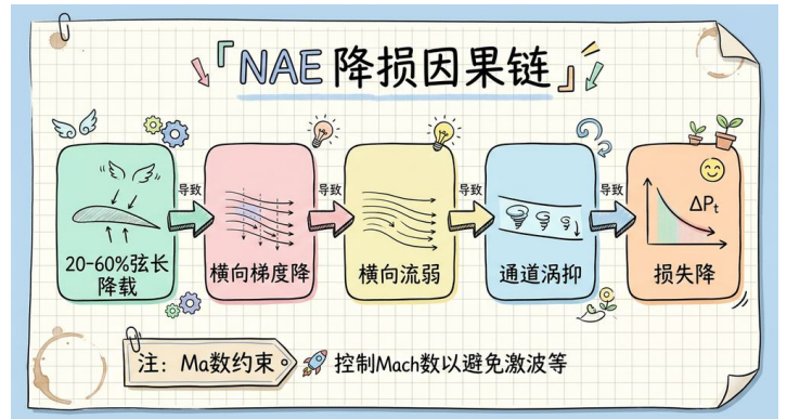
causal chain NAE降损机理链(须绑Ma)
