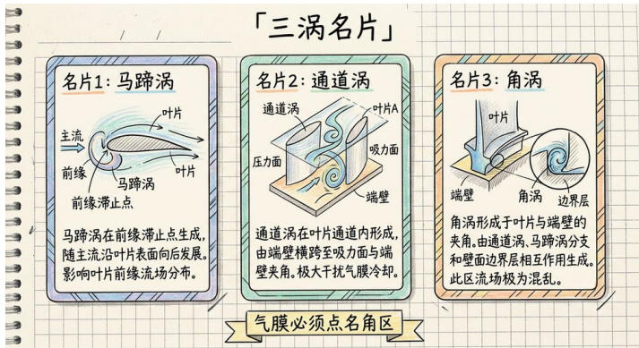
three vortex cards 马蹄/通道/角涡名片
