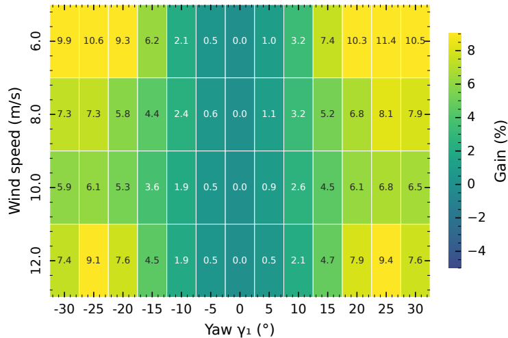
Gain matrix (yaw \times wind)
