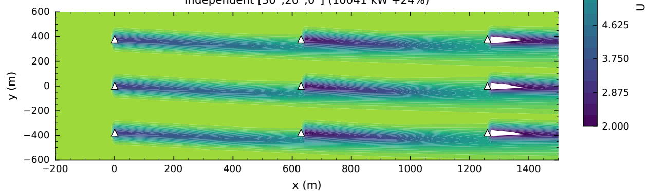
Independent [30^\circ, 20^\circ, 0^\circ] (10041 kW +24%)
