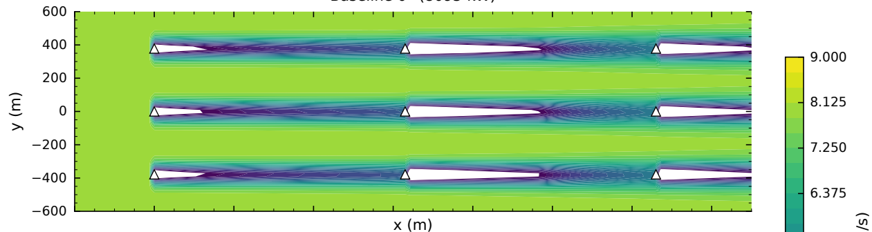
Independent [30^\circ, 20^\circ, 0^\circ] (10041 kW +24%)
