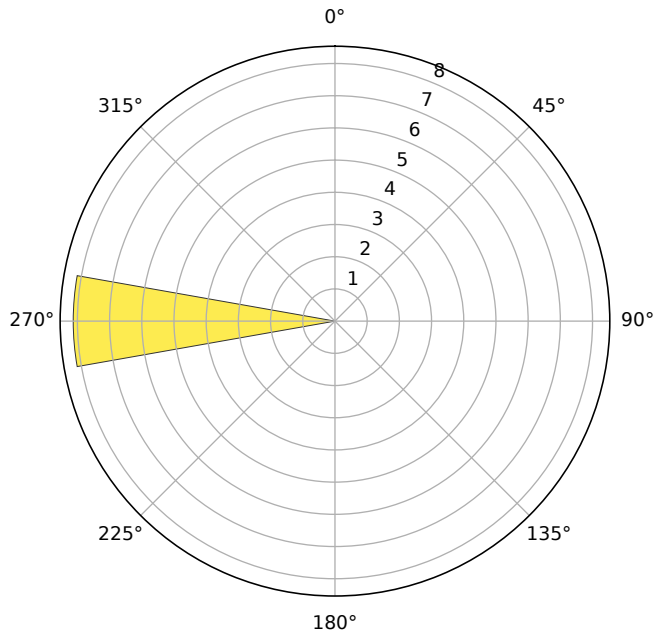
Optimal gain vs wind direction (8 m/s)
