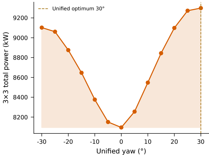
Array unified yaw sweep
