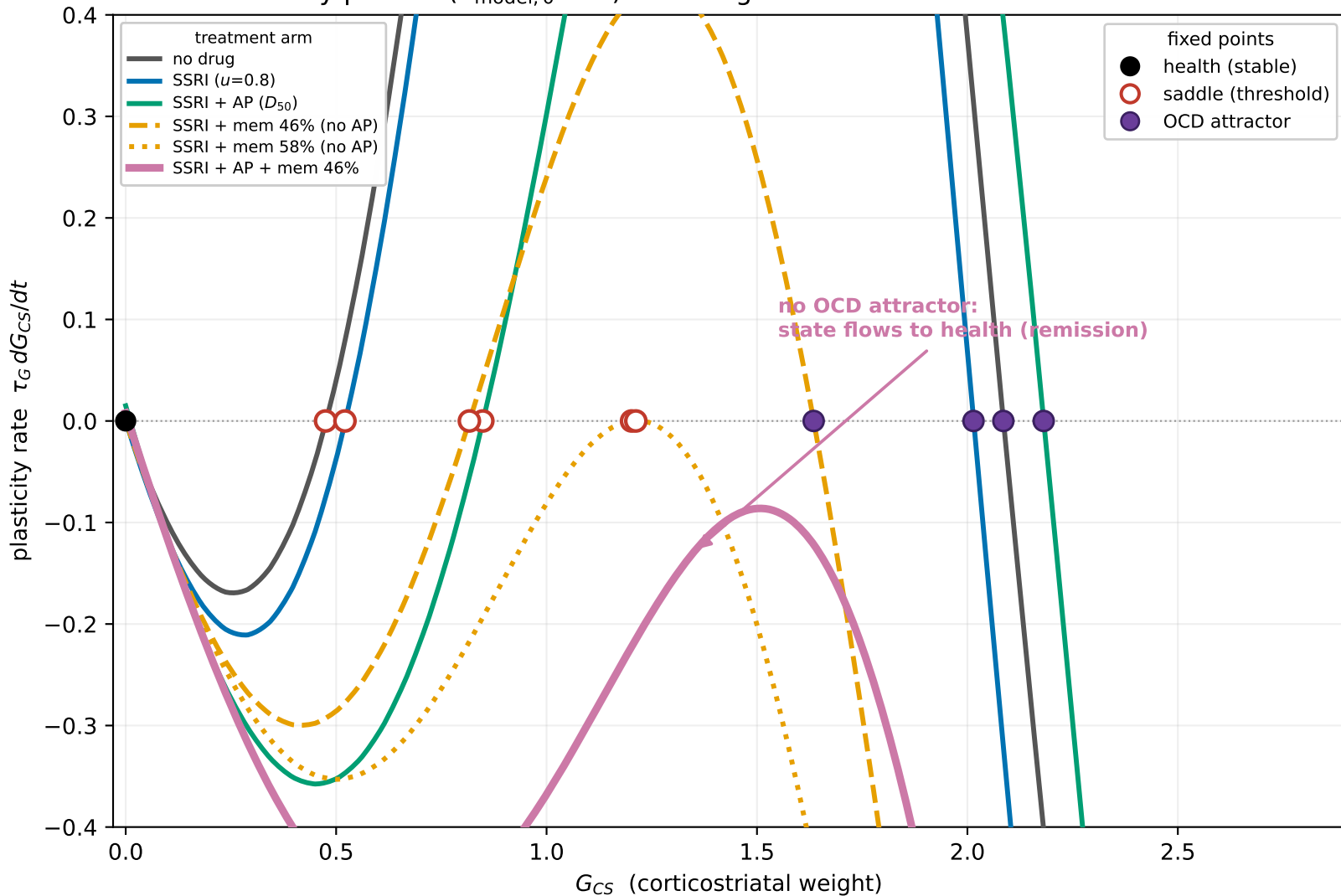
Refractory patient ( Y_{\text{model},0}=32 ): stacking mechanisms annihilates the attractor
