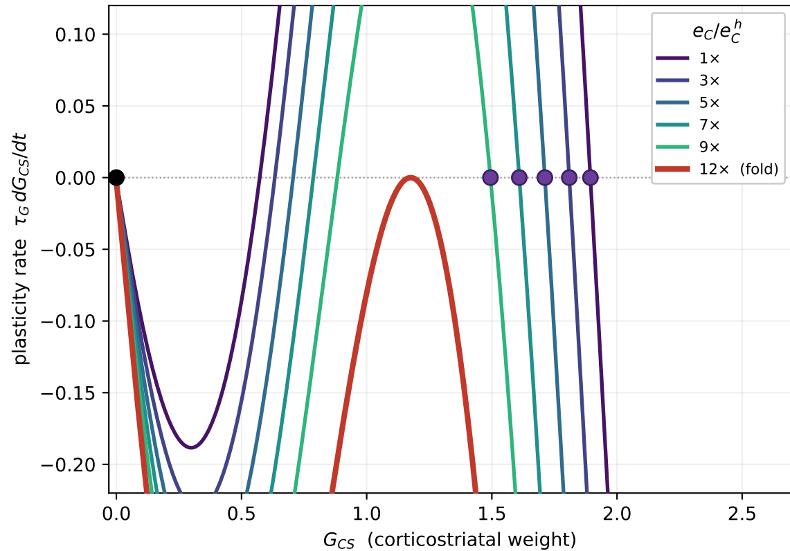
(a) Y_{\text{model},0}=28 : attractor annihilates only at e_c=12\times baseline
