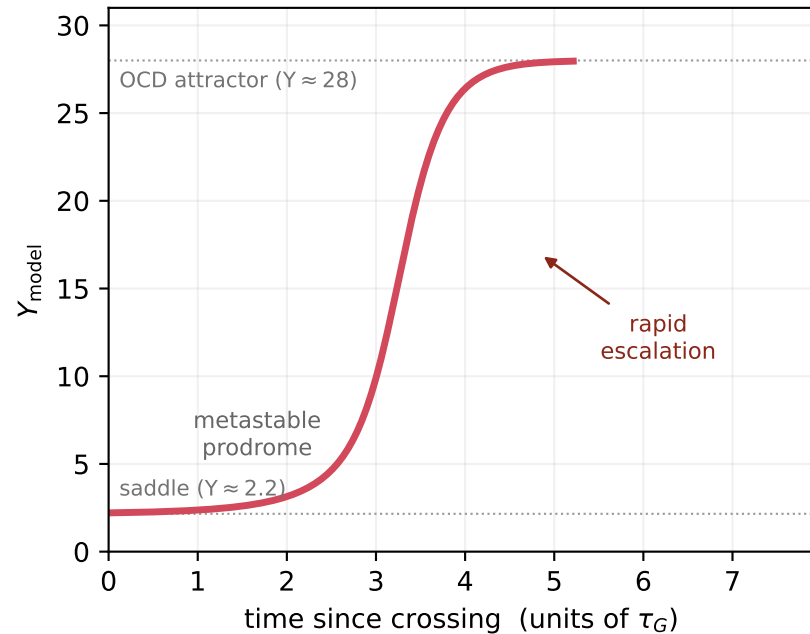
(c) onset once past the tipping point
