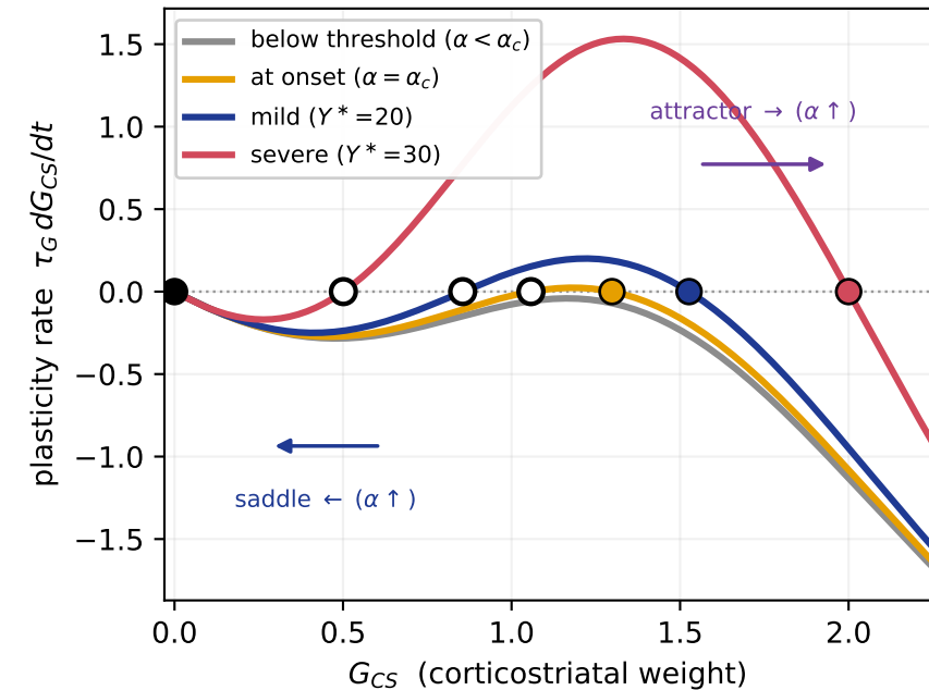
(a) the landscape as vulnerability \alpha grows
