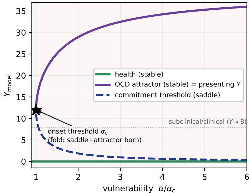
(b) onset threshold and the two branches
