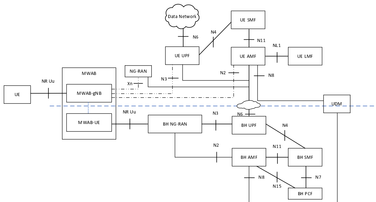
Figure S.2-1: Architecture for MWAB operation support - non-roaming with one PLMN
