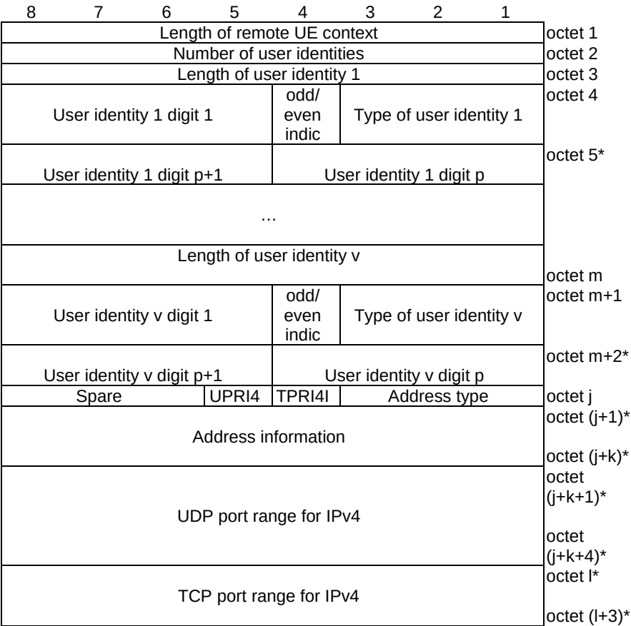
Figure 9.9.4.20.2: Remote UE context
