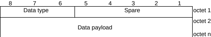
Figure 9.9.3.74.3: Data container IE for Data type "SMS"
