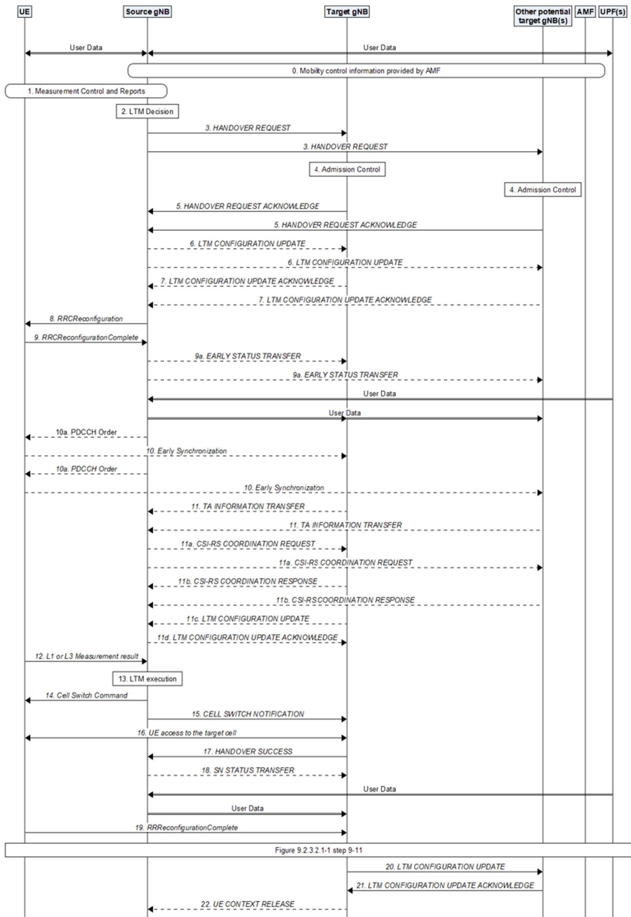
Figure 9.2.3.5.2-2. Signalling procedure for inter-gNB LTM
