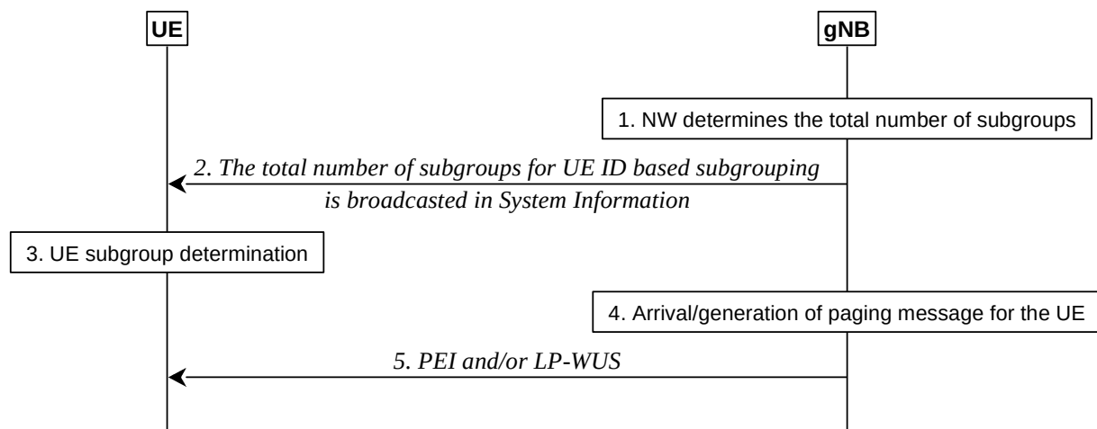
Figure 9.2.5-2: Procedure for UE ID based subgrouping
