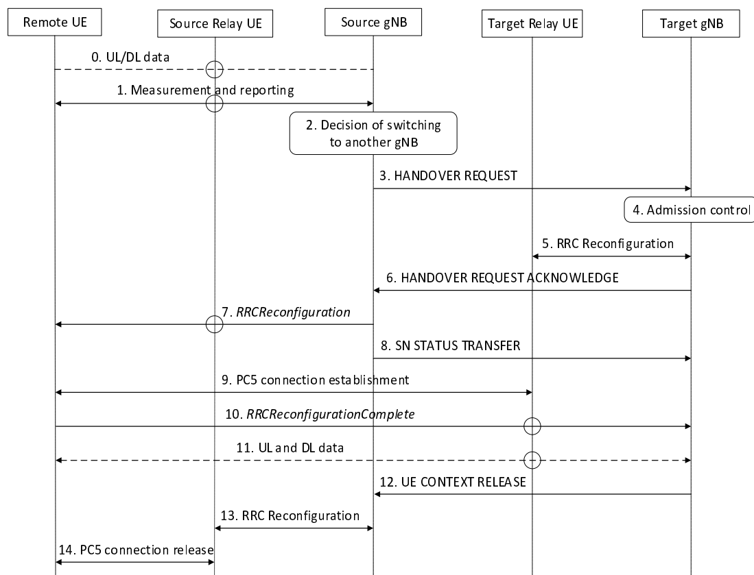
Figure 16.12.6.3-2: Procedure for L2 U2N Remote UE inter-gNB switching from single-hop indirect to single-hop indirect path via a target L2 U2N Relay UE in RRC_CONNECTED
