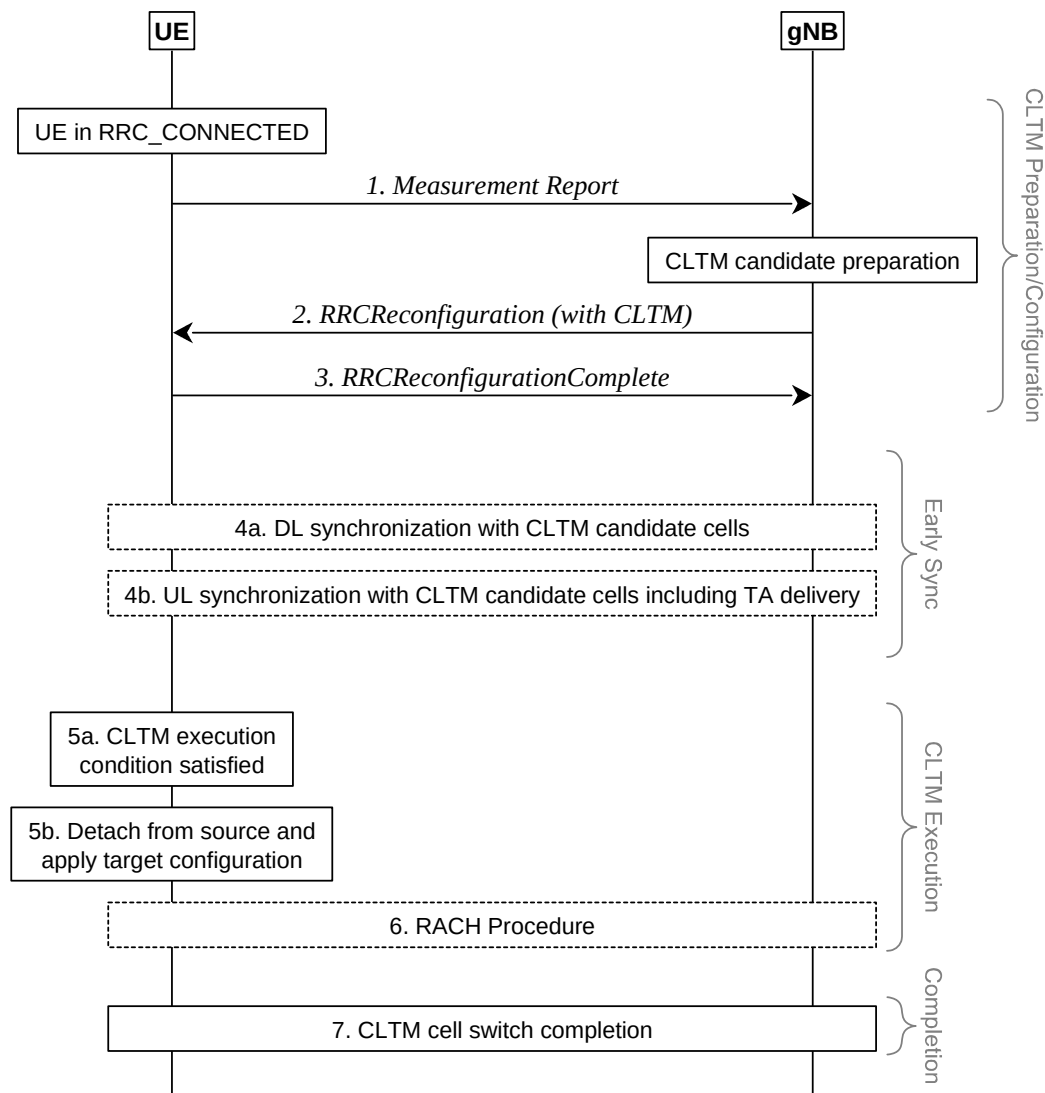
Figure 9.2.3.7.1-1. Signalling procedure for CLTM
