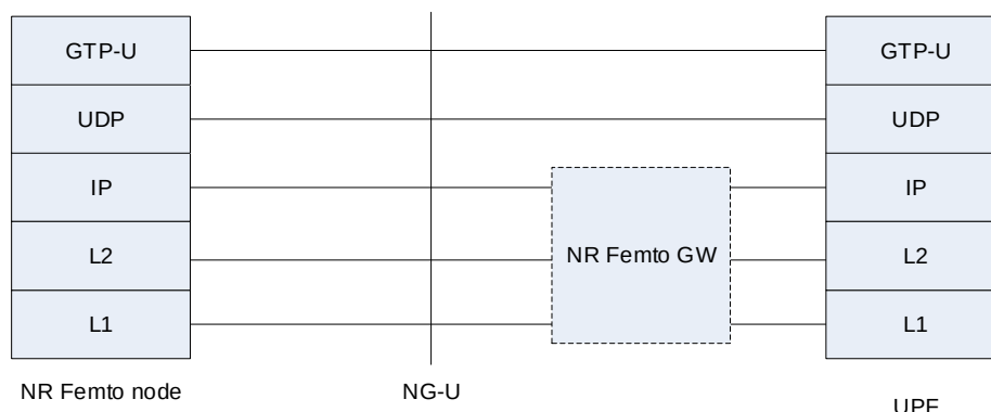
Figure 4.10.3.1-1: User plane for NG Interface between NR Femto node and UPF
