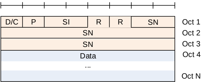
Figure 6.2.2.4-2: AMD PDU with 18 bit SN (No SO)
