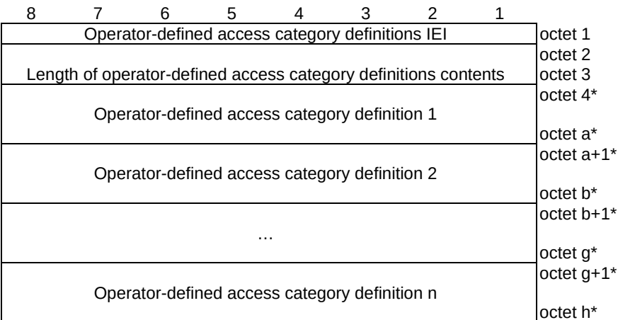
Figure 9.11.3.38.1: Operator-defined access category definitions information element
