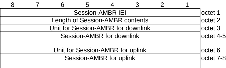
Figure 9.11.4.14.1: Session-AMBR information element
