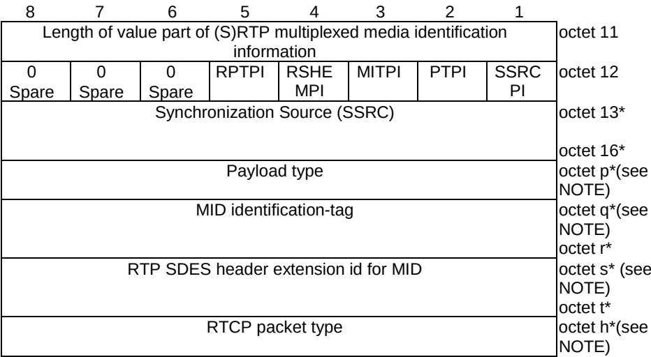
Figure 9.11.4.13.6: (S)RTP multiplexed media identification information entry
