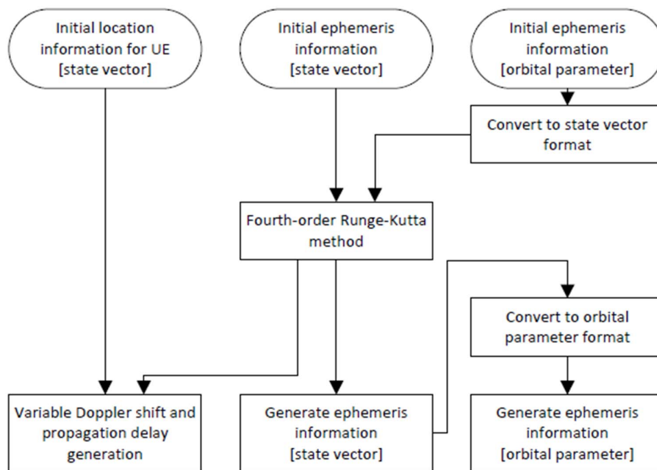
Figure G.1-2: Calculation flow for time varying channel conditions by Fourth-order Runge-Kutta method
