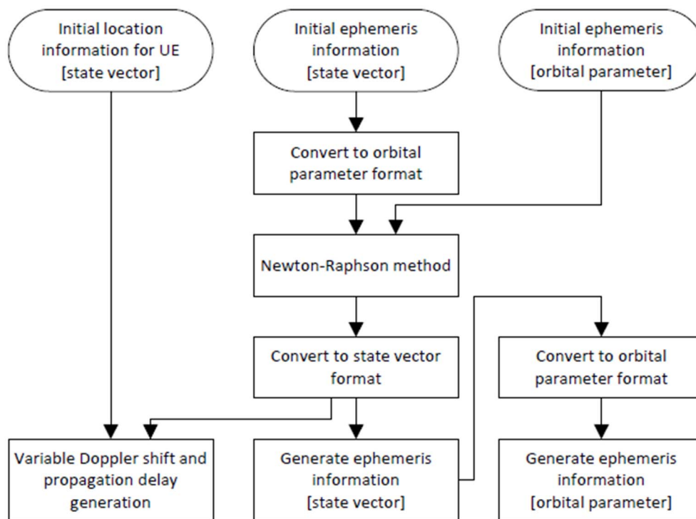
Figure G.1-1: Calculation flow for time varying channel conditions by Newton-Raphson method
