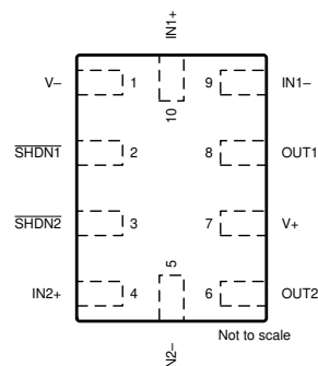
Figure 5-9. TLV9062S RUG Package, 10-Pin X2QFN (Top View)
