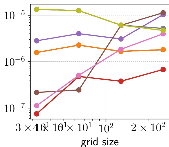
Relative error
