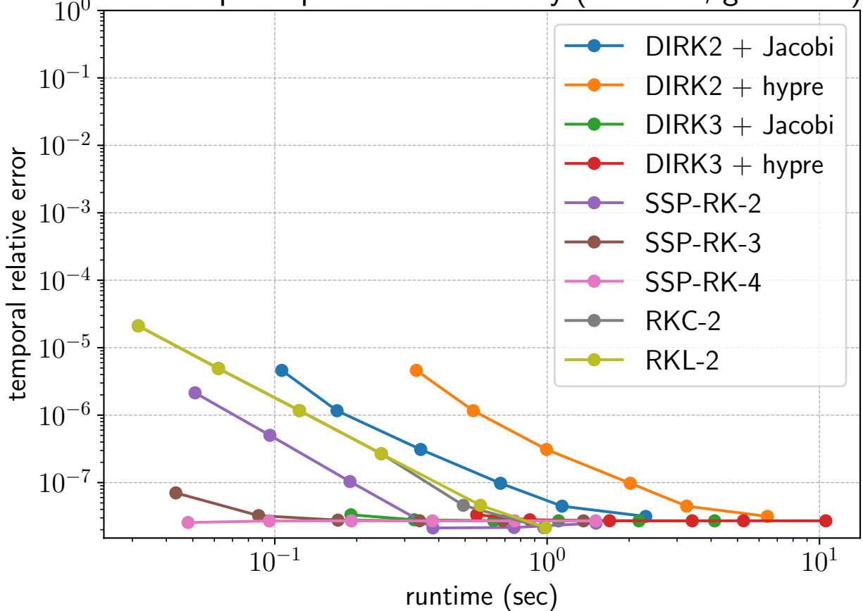
Fixed step computational efficiency ( kx = 0.1 , grid = 64)
