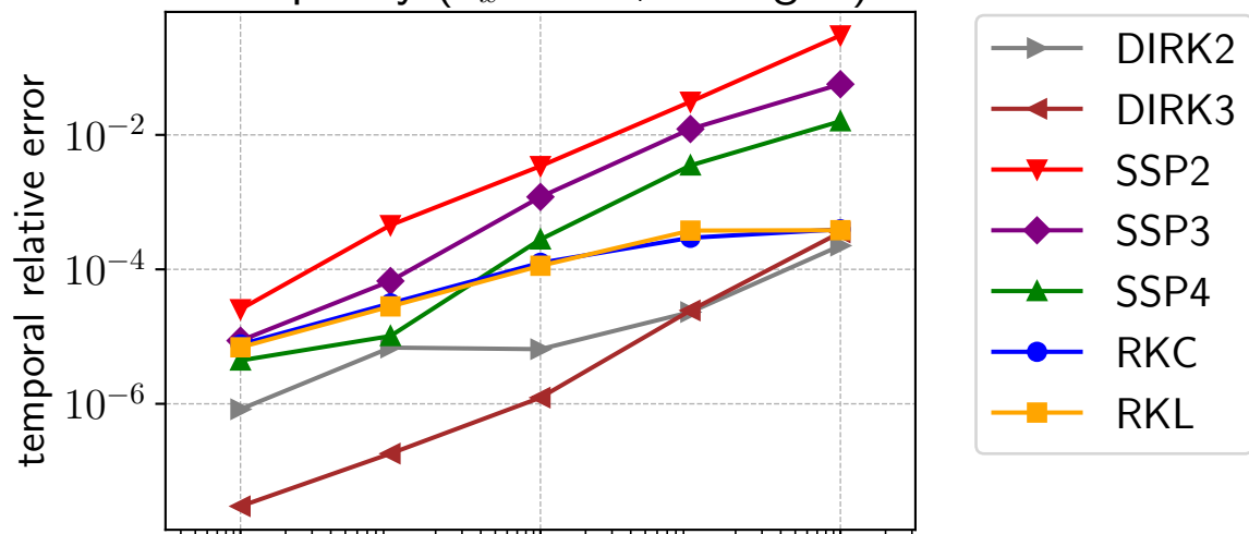
Adaptivity ( \nu_x = 1.0 , 128^2 grid)
