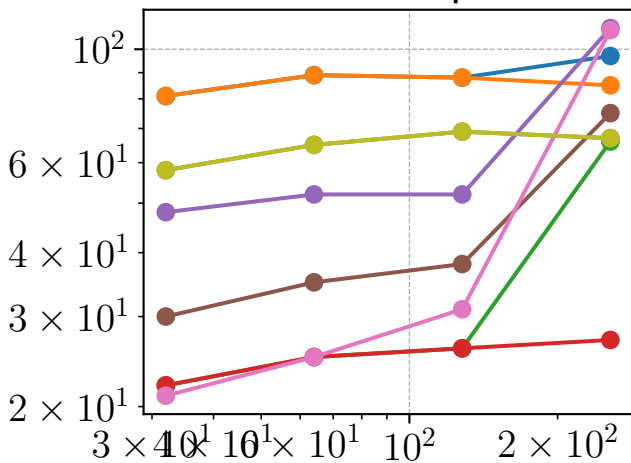
Relative error
