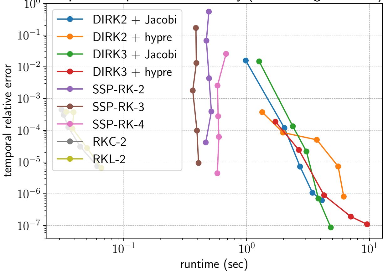
Adaptive computational efficiency ( kx = 1.0 , grid = 256)
