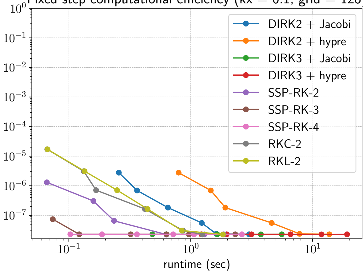
Fixed step computational efficiency ( kx = 0.1 , grid = 128)
