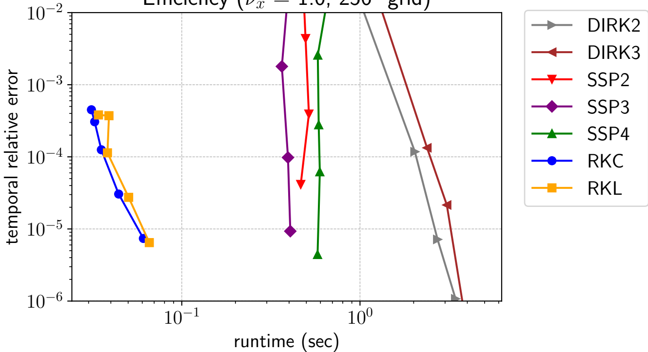
Efficiency ( \nu_x = 1.0 , 256^2 grid)
