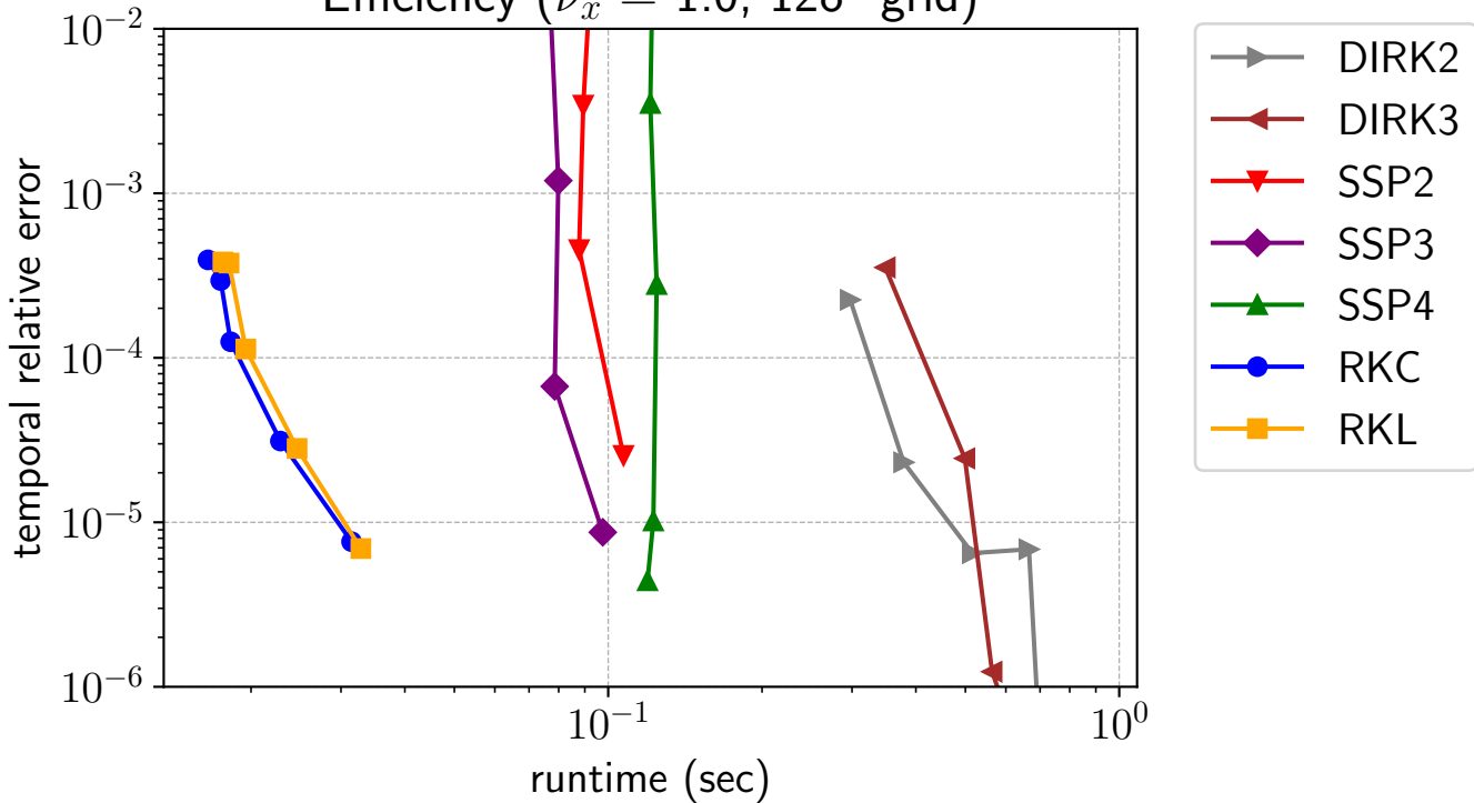
Efficiency ( \nu_x = 1.0 , 128^2 grid)
