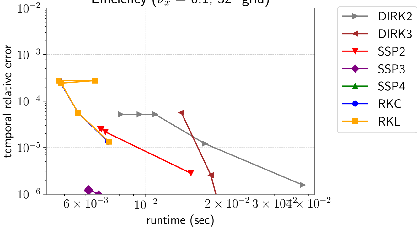
Efficiency ( \nu_x = 0.1 , 32^2 grid)
