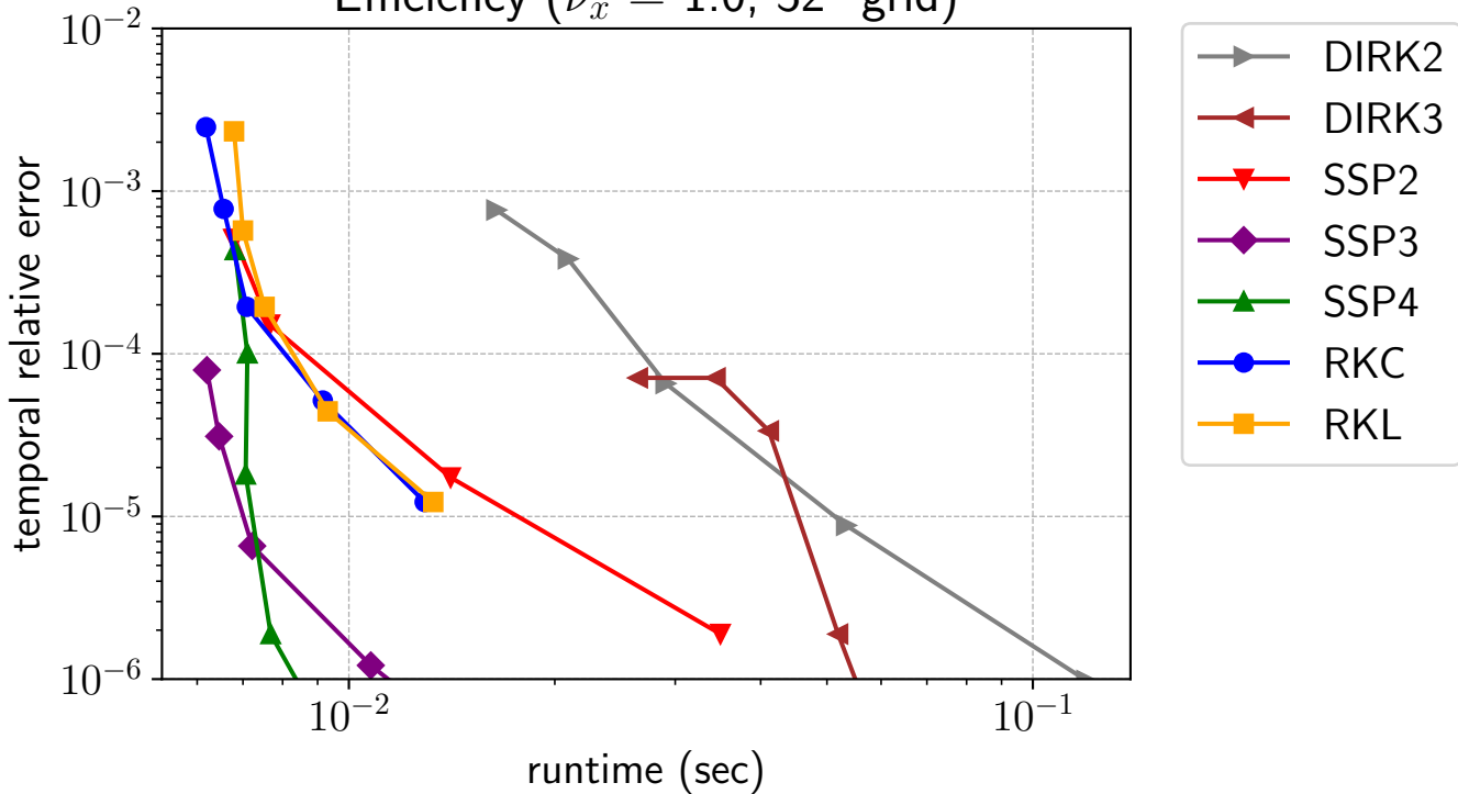
Efficiency ( \nu_x = 1.0 , 32^2 grid)
