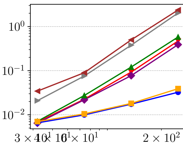
Runtime
