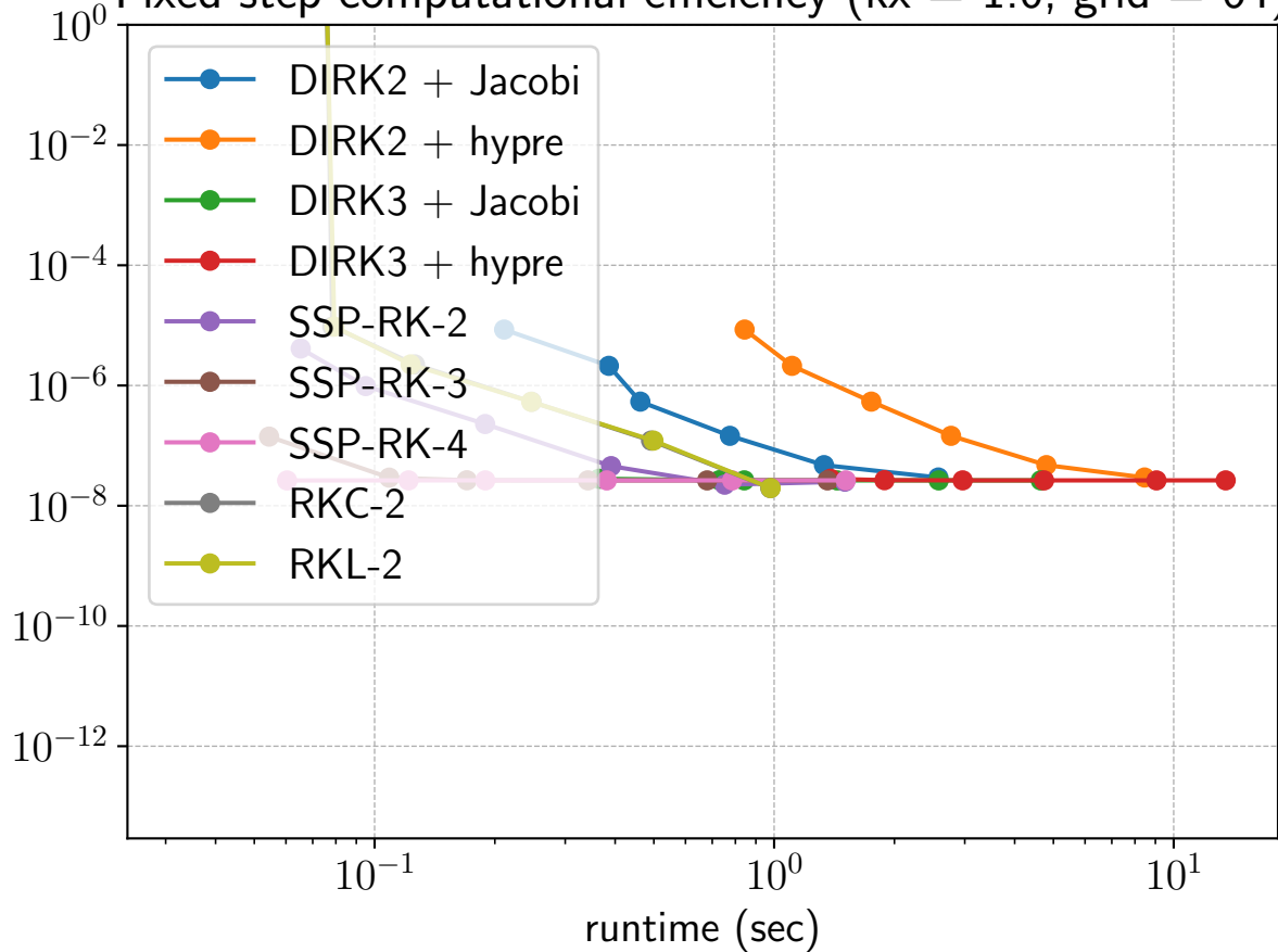
Fixed step computational efficiency ( k_x = 1.0 , \text{grid} = 64 )
