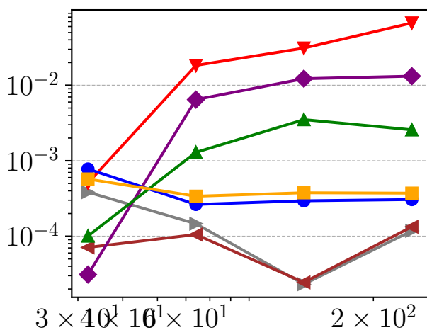
Relative error
