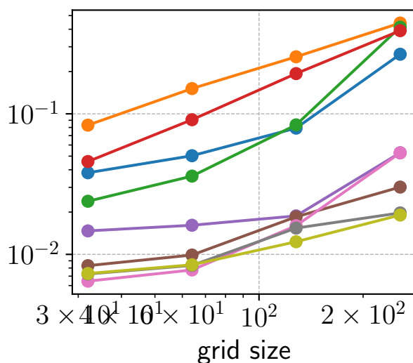
Runtime
