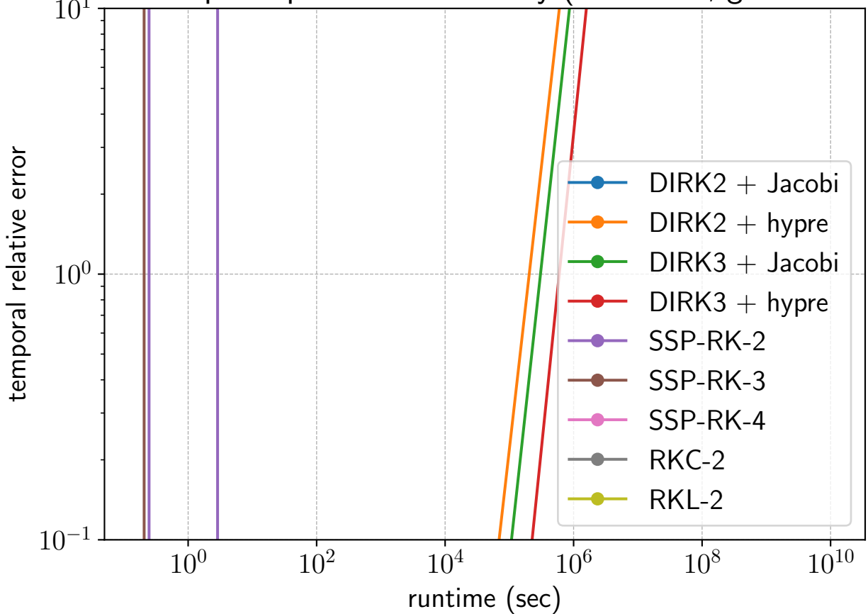
Fixed step computational efficiency ( kx = 10.0 , grid = 256)
