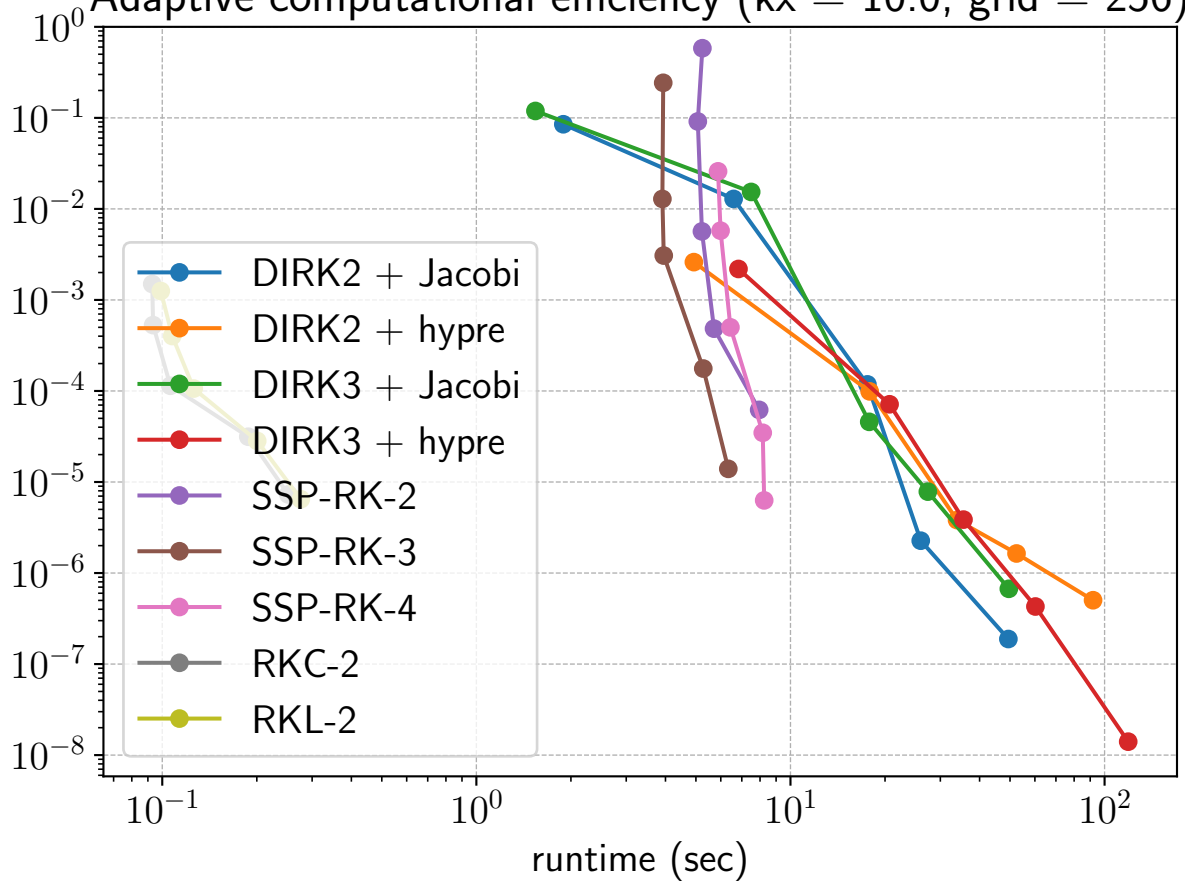
Adaptive computational efficiency ( kx = 10.0 , grid = 256)
