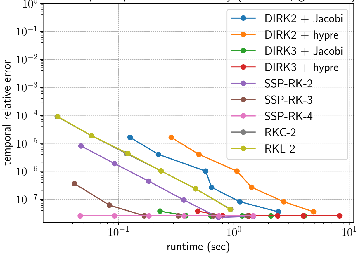
Fixed step computational efficiency ( kx = 1.0 , grid = 32)
