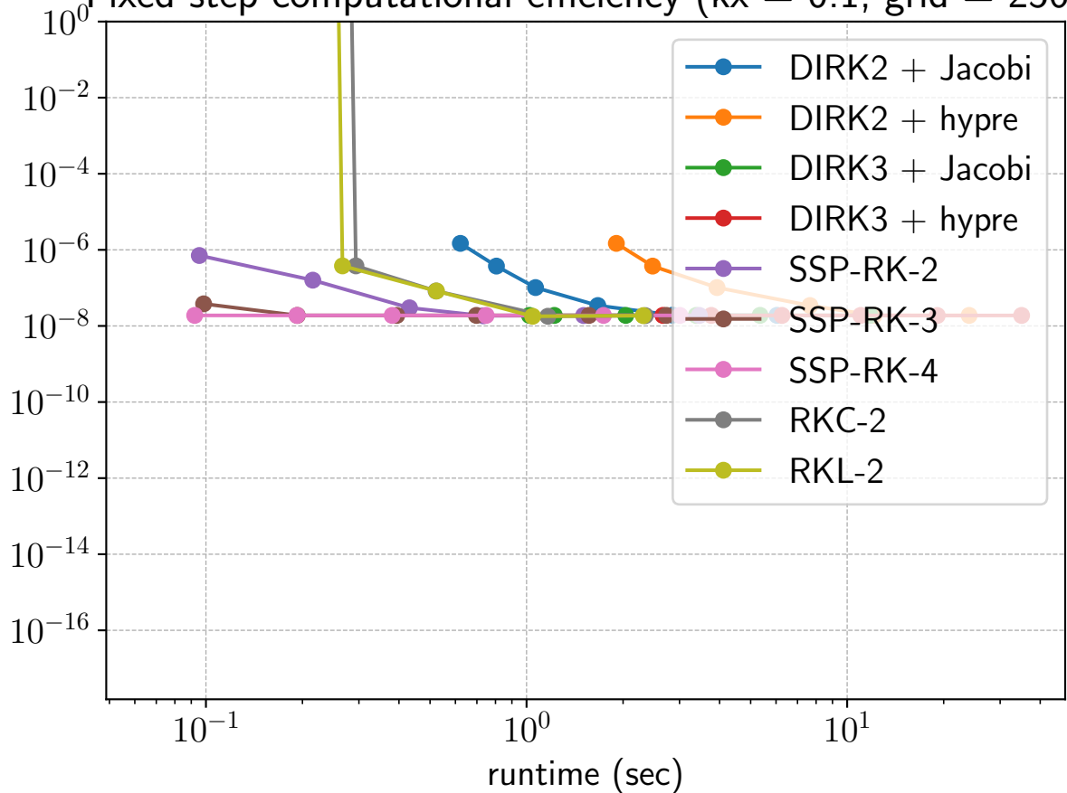
Fixed step computational efficiency ( kx = 0.1 , grid = 256)
