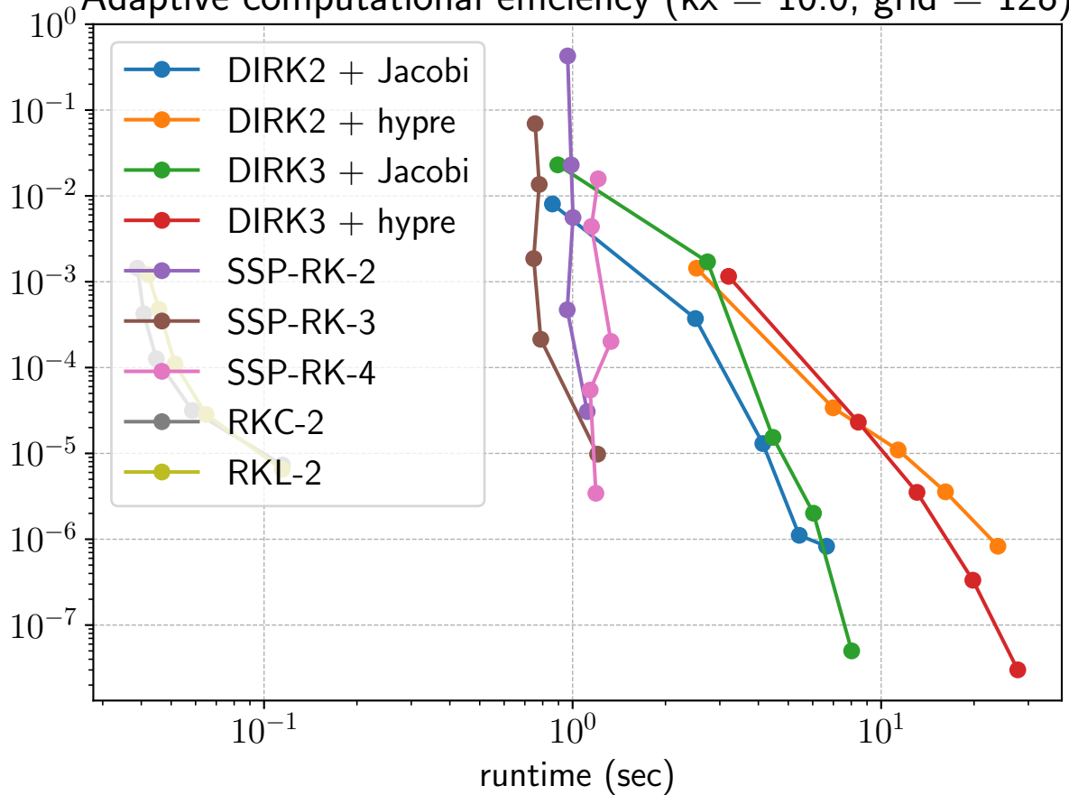
Adaptive computational efficiency ( kx = 10.0 , grid = 128)
