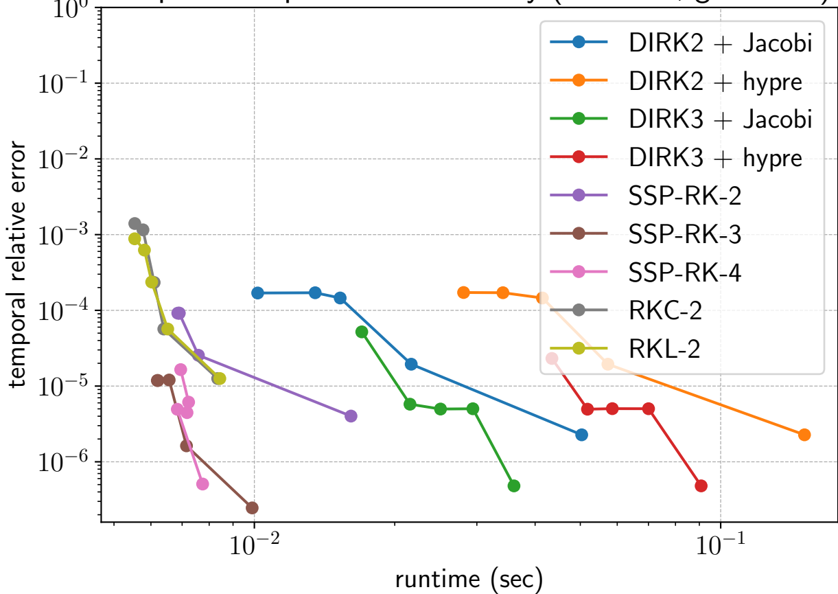
Adaptive computational efficiency ( kx = 0.1 , grid = 64)
