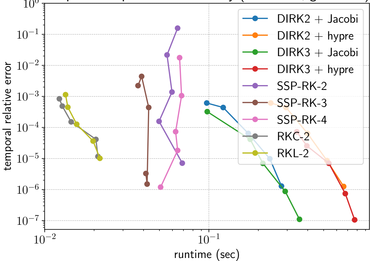
Adaptive computational efficiency ( kx = 10.0 , grid = 32)
