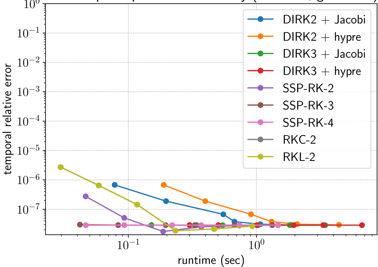
Fixed step computational efficiency ( kx = 0.1 , grid = 32)
