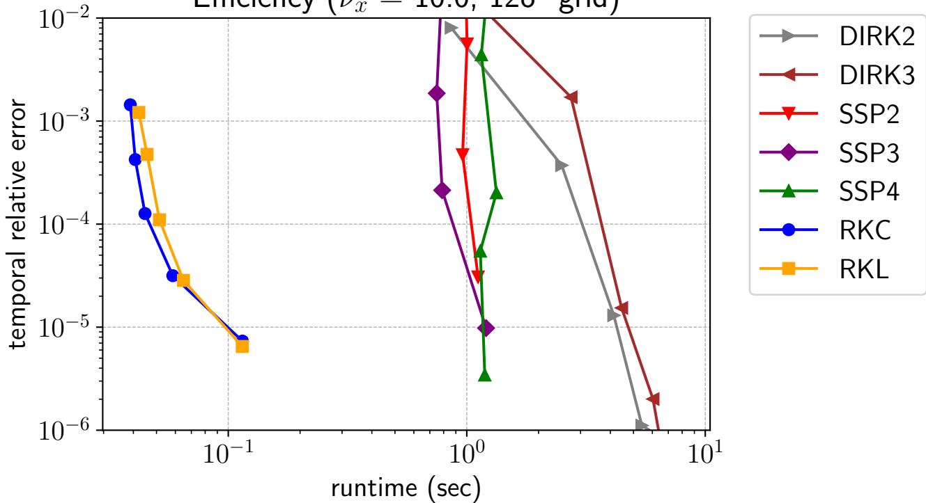
Efficiency ( \nu_x = 10.0 , 128^2 grid)
