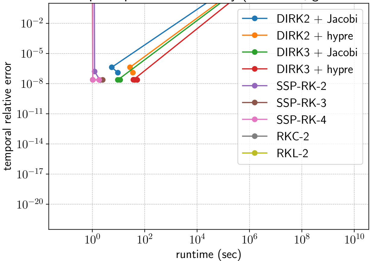
Fixed step computational efficiency ( kx = 10.0 , grid = 128)
