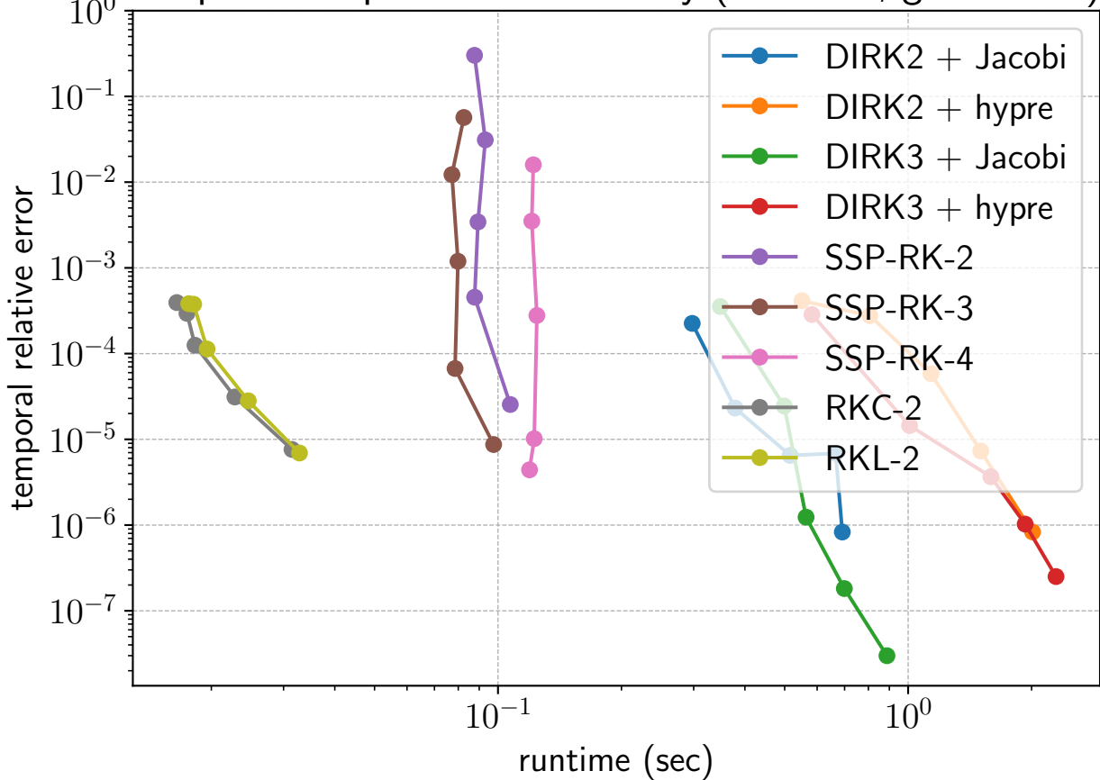
Adaptive computational efficiency ( kx = 1.0 , grid = 128)
