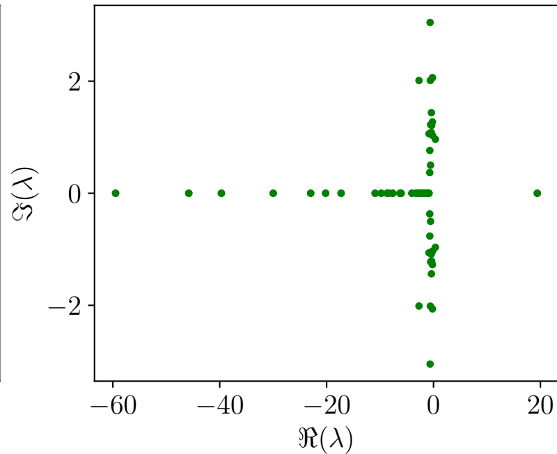
reaction \lambda_{max}
