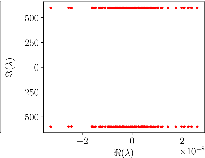
advection \lambda_{max}
