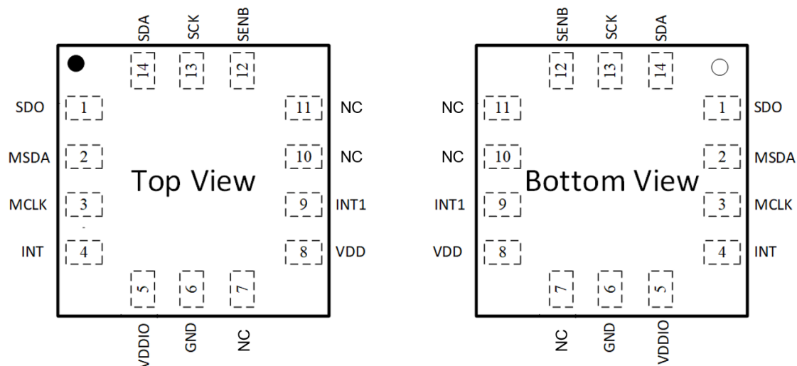
Figure 4: The pin out view of SH3001
