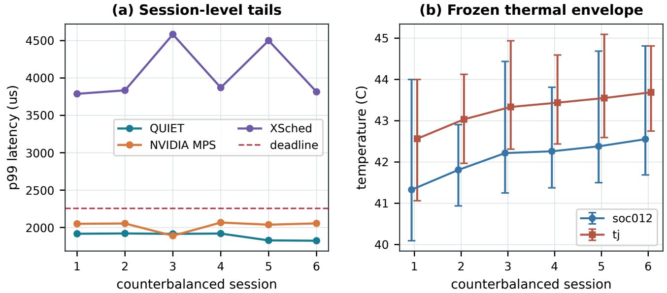
Figure 6: Independent-session stability. Panel (a) reports each session’s p99 against the fixed deadline. Panel (b) reports mean soc012 and tj temperatures with observed minimum–maximum bars. Thermal conditions define admissibility; they are not used to rescale latency.
