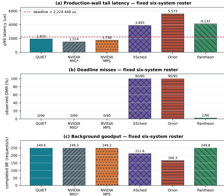
Figure 8: Fixed-roster directional ImageNet gate. Every panel repeats QUIET, NVIDIA MIG, NVIDIA MPS, XSched, Orion, and Pantheon in the same order. All rows consume the same 90 labelled inputs, operational arrivals, and 2,224.448 \mu s deadline. This one-session coverage gate is not a formal rank; MIG uses its valid BE-capable layout, with the critical DAG on 2g and the background tenant on the isolated 1g instance.
