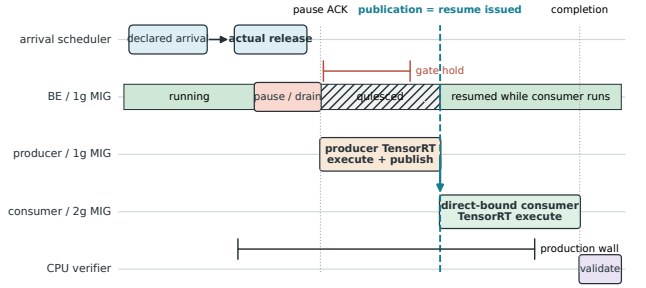
Figure 3: QUIET’s request lifecycle. The operational release precedes gate acquisition, so queue and drain delay remain inside the production wall. Producer publication is the protection boundary: resume is issued before checksum and output validation, and best-effort work overlaps the consumer.
