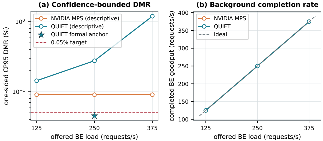
Figure 7: Same-workload offered-load sweep. Hollow markers are descriptive three-session points (3,300 requests/point) and are not thermal normalized. The star is the separate six-session, thermal-qualified QUIET anchor at 250 requests/s. No hollow point is used for ranking.
