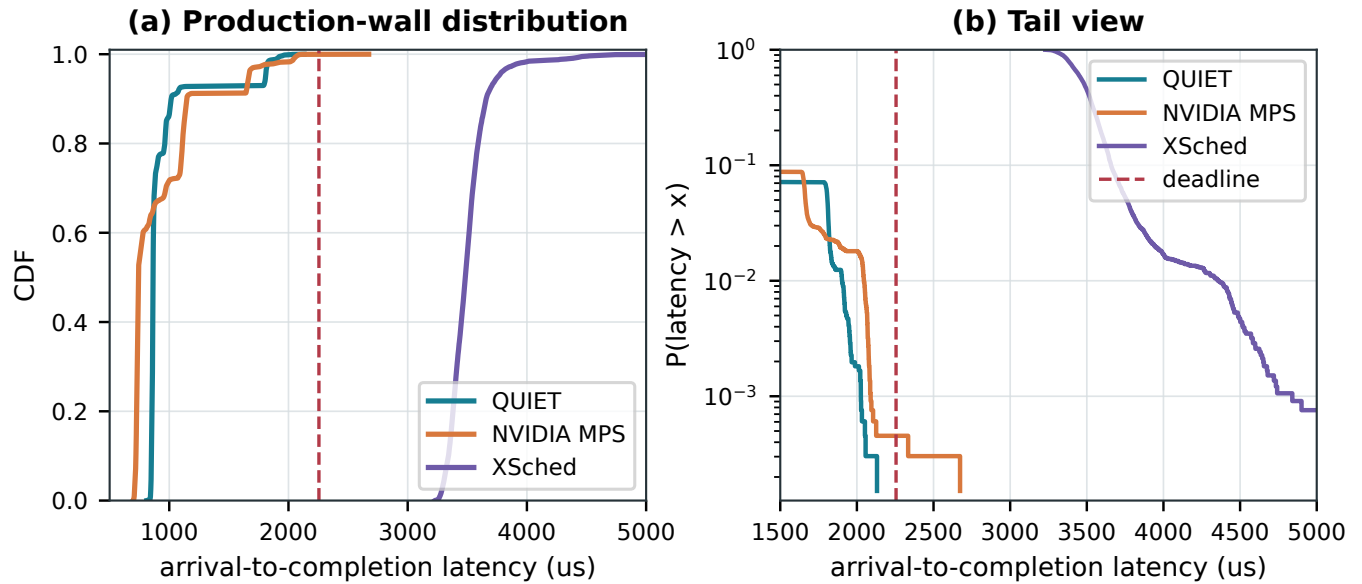
Figure 5: Request-level latency in the six-session thermal-normalized ImageNette campaign (6,600 requests/system). The left panel shows the full CDF; the right isolates the tail on a logarithmic survival axis. The dashed line is the frozen 2,255.483 \mu s production-wall deadline.
