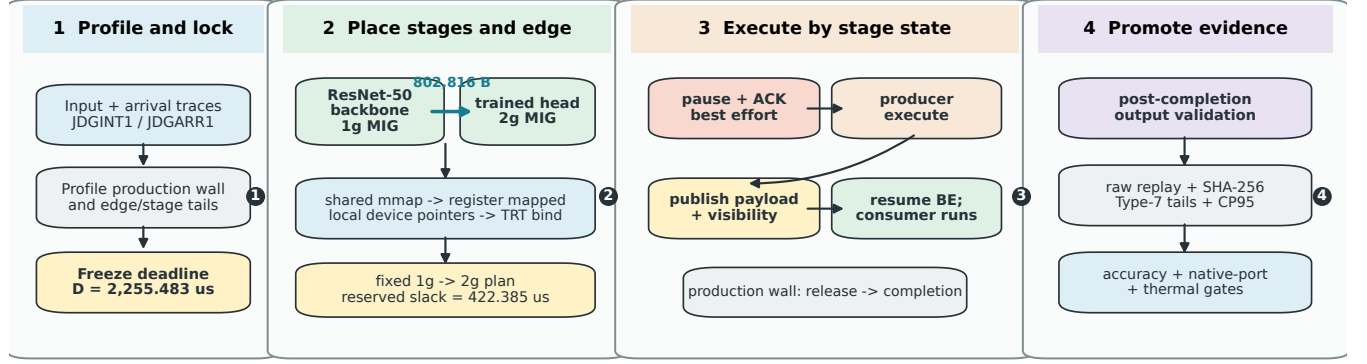
Figure 1: The architecture and procedure of QUIET. The planner freezes a workload-specific deadline, places the two validated stages and their activation edge, and serializes the resulting contract. At runtime, best-effort work is protected only through producer publication. Accuracy, raw-replay, native-port, and thermal gates determine which results may be promoted. The current production path is a two-stage chain, not a general-DAG runtime.
