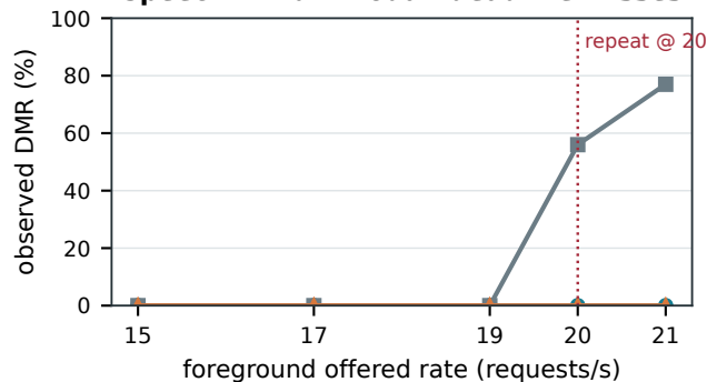
Speech + Multimodal: deadline misses
