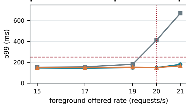
Speech + Multimodal: production-wall p99
