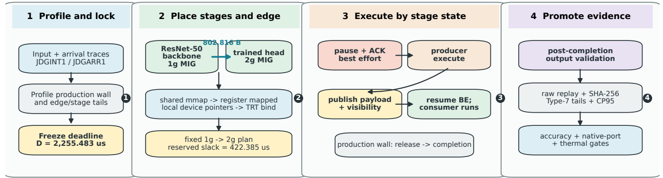
Jetson AGX Thor: isolated MIG execution/local allocations over physically shared coherent SoC DRAM
