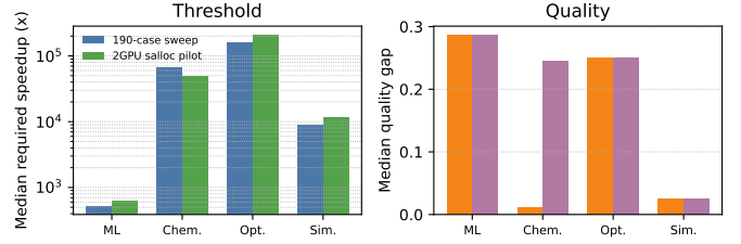
Fig. 8: Official 190-case sweep versus the 96-case bundled salloc pilot. The pilot uses two A100 GPUs inside one allocation and reproduces the same qualitative conclusion: every workload family remains outside the current advantage region, but the required hardware improvement differs by family.
