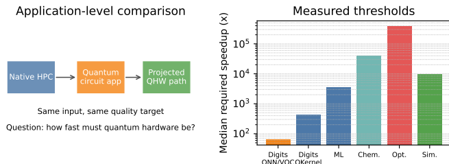
Fig. 1: Application-level comparison target. The key comparison is not simulator versus simulator. The key comparison is native application execution versus quantum-circuit application execution and projected quantum hardware execution.
