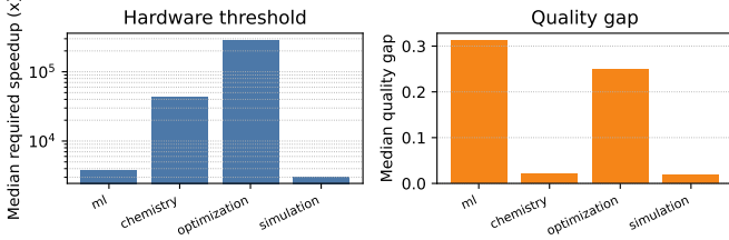
Fig. 4: Large practical suite over 3,552 cases. Each bar compares the selected native HPC-style baseline with a quantum-circuit application path simulated through cuQuantum. All families currently require faster projected quantum execution, but the threshold differs by application class.
