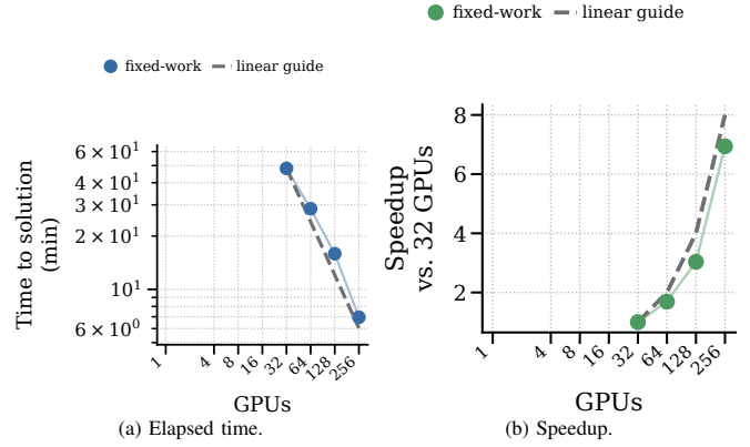
Fig. 6: Strong scaling of the fixed 7,104-case application suite. Both subfigures keep the full 1/4/8/16/32/64/128/256 GPU labels, while measured fixed-work markers begin at 32 GPUs. The direct run reduces time-to-solution from 48 minutes 14 seconds on 32 GPUs to 6 minutes 58 seconds on 256 GPUs. Dashed lines are visual guides, not additional measured runs.
