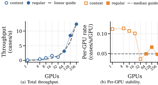
Fig. 5: Weak scaling from 1 to 256 GPUs. Both subfigures keep the full 1/4/8/16/32/64/128/256 GPU labels. Hollow markers denote context runs with smaller per-GPU work; solid markers denote the regular large-profile weak-scaling regime. Dashed lines are visual guides, not additional measured runs.
