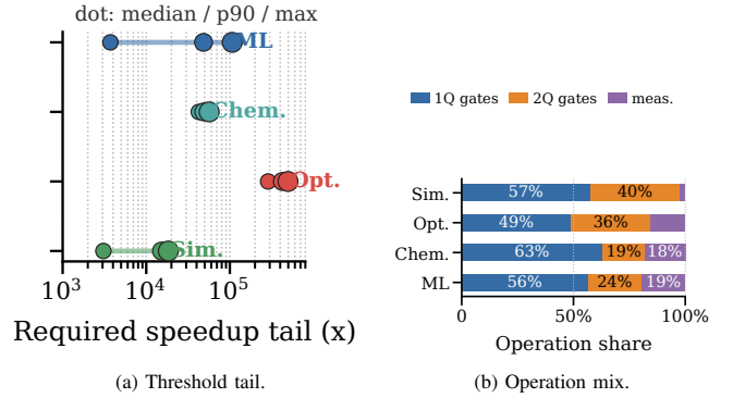
Fig. 8: Tail and circuit pressure by workload. The left plot shows median, 90th percentile, and maximum threshold pressure; the right plot separates one-qubit, two-qubit, and measurement pressure after the fixed simulation floor is removed.
