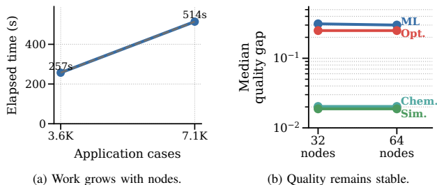
Fig. 10: Larger-workload gate on 64 Perlmutter GPU nodes. The 64-node run completes 7,104 cases in 514 seconds with empty stderr logs. The larger run preserves the workload-level quality interpretation, so the extra cases increase evidence coverage rather than changing the advantage conclusion.
