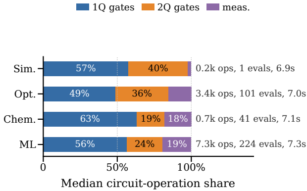
Fig. 8: Circuit-operation pressure by workload. The measured circuit path spends work differently across families: ML is dominated by feature-map evaluations, optimization by repeated QAOA grids, chemistry by VQE term evaluation, and simulation by fewer but state-evolution-heavy circuits.
