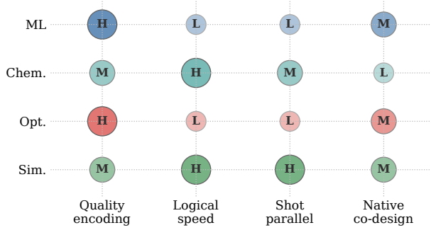
Fig. 14: Architecture focus implied by the measured frontier and bottleneck taxonomy. L/M/H labels summarize where future-system effort is likely to matter first for each workload family.
