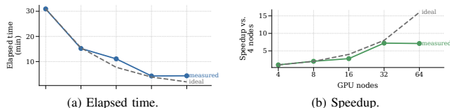
Fig. 12: Strong scaling of the fixed 3,552-case application suite. The run reduces time-to-solution from 30 minutes 55 seconds on four nodes to about 4 minutes 20 seconds on 32–64 nodes, where task granularity and case imbalance become the limit.
