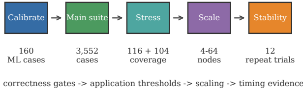
Fig. 5: Completed Perlmutter evidence campaign. The figure separates correctness, application coverage, scaling, and timing evidence instead of compressing the evaluation plan into a table.
