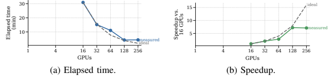
Fig. 12: Strong scaling of the fixed 3,552-case application suite. The run reduces time-to-solution from 30 minutes 55 seconds on 16 GPUs to about 4 minutes 20 seconds on 128–256 GPUs, where task granularity and case imbalance become the limit.
