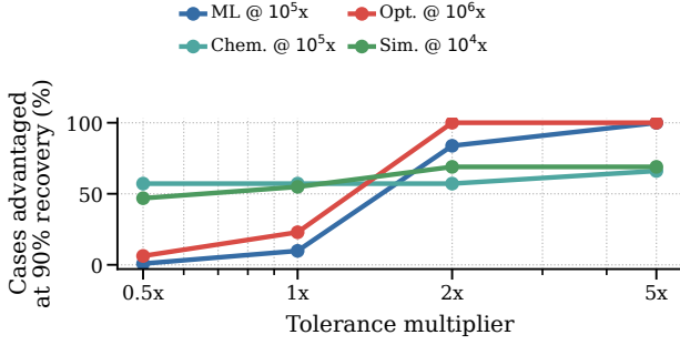
Fig. 14: Tolerance sensitivity of the advantage frontier. The same measured cases can be reinterpreted under stricter or looser quality budgets; this changes quality-limited ML and optimization much more than speed-bound chemistry.
