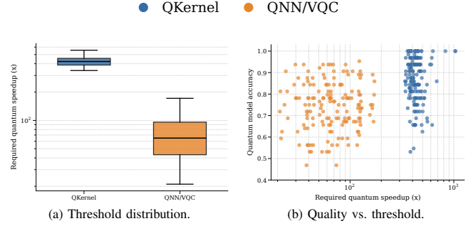
Fig. 6: Expanded digits results over 160 cases. The quantum-kernel path often reaches useful accuracy but needs hundreds of times faster execution, while QNN/VQC has a lower threshold but usually lower quality.
