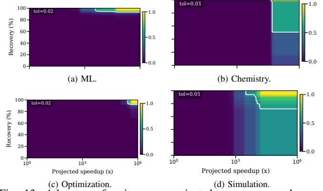
Fig. 13: Advantage frontier over projected quantum speedup and quality-gap recovery. Color shows the fraction of measured cases in each family that would enter the advantage region under that hypothetical hardware and algorithmic improvement. The contour marks the 50% frontier when it appears.
