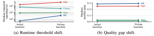
Fig. 9: Native baseline stress test. The slope view shows how each workload moves when the native path is strengthened, instead of hiding the shift inside grouped bars. Strengthening the native side makes the ML threshold 6.6\times larger and the optimization threshold 2.3\times larger than the initial native-baseline sweep.
