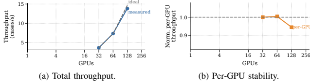
Fig. 11: Weak scaling of the comparable large-profile application suite. Total throughput grows nearly linearly from 32 to 128 GPUs while normalized per-GPU throughput remains close to the 32-GPU reference.
