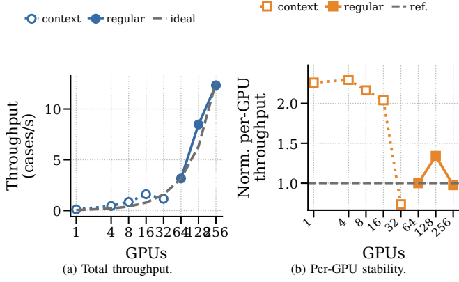
Fig. 5: Weak scaling from 1 to 256 GPUs. Hollow markers show completed 1–32 GPU context runs used to expose low-end launch behavior; solid markers show the regular large-profile weak-scaling ladder from 64 to 256 GPUs. The regular 64/128/256-GPU runs complete 1,776, 3,552, and 7,104 cases, respectively.
