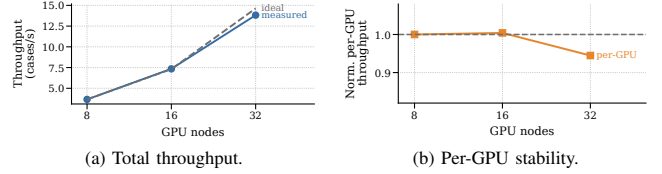
Fig. 11: Weak scaling of the comparable large-profile application suite. Total throughput grows nearly linearly from 8 to 32 nodes while normalized per-GPU throughput remains close to the 8-node reference.
