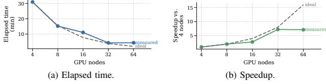
Fig. 12: Strong scaling of the fixed 3,552-case application suite. The run reduces time-to-solution from 30 minutes 55 seconds on four nodes to about 4 minutes 20 seconds on 32–64 nodes, where task granularity and case imbalance become the limit.
