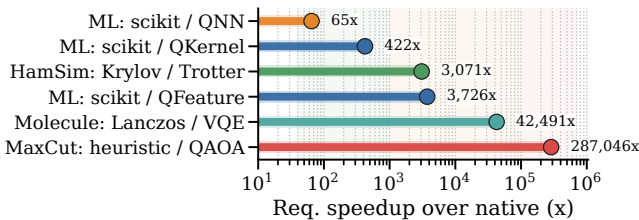
Fig. 1: Required speedup for each native/quantum pair. The left side of each label names the native HPC/ML baseline and the right side names the quantum-circuit path.
