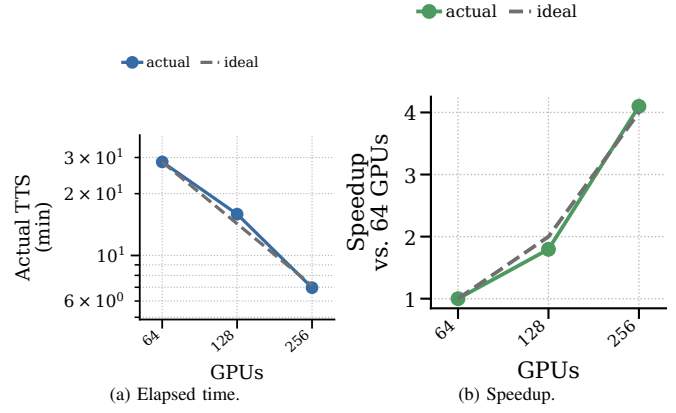
Fig. 6: Strong scaling of the fixed 7,104-case application suite. Both subfigures use only direct fixed-suite regular-queue runs on 64, 128, and 256 GPUs. The measured run reduces time-to-solution from 28 minutes 33 seconds on 64 GPUs to 6 minutes 58 seconds on 256 GPUs.
