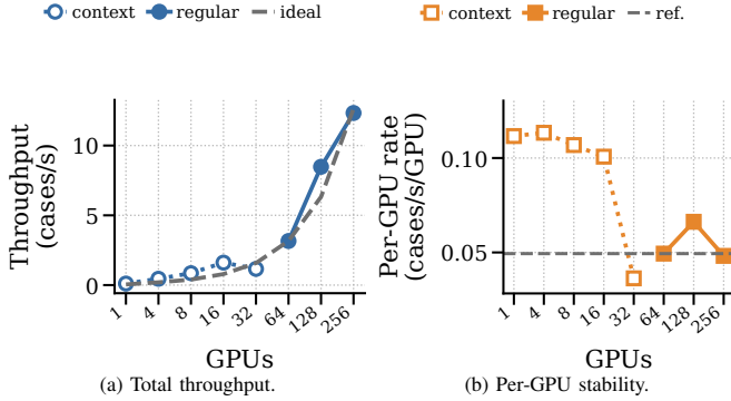
Fig. 5: Weak scaling from 1 to 256 GPUs. Hollow markers keep the completed 1–32 GPU context ladder on the same axis; solid markers show the regular large-profile weak-scaling ladder from 64 to 256 GPUs. The right plot reports raw per-GPU rate, with the dashed line marking the regular-ladder median, so the low-end context runs are visible but not treated as the same weak-scaling regime.
