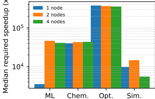
Threshold stability
