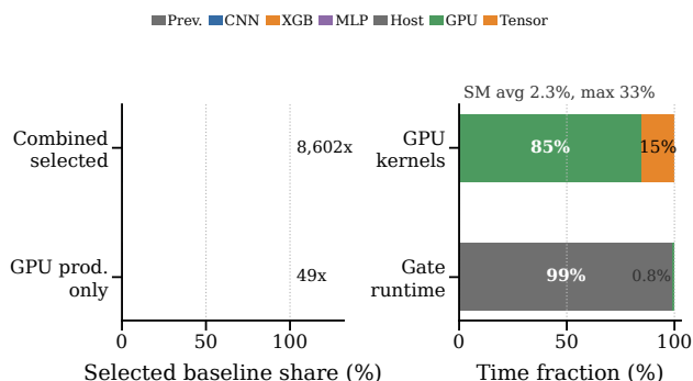
Fig. 8: ML production-native and profiling gate. PyTorch AMP and XGBoost candidates reach native-level quality, but the small digits task remains dominated by previous microsecond baselines and by host orchestration in the profiled GPU gate.
