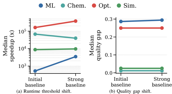
Fig. 7: Native baseline stress test. The slope view shows how each workload moves when the native path is strengthened, instead of hiding the shift inside grouped bars. Strengthening the native side makes the ML threshold 6.6\times larger and the optimization threshold 2.3\times larger than the initial native-baseline sweep.
