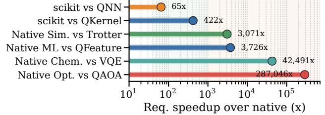
Fig. 1: Required speedup of each quantum-circuit path over its native counterpart. Workload definitions are in Table II.
