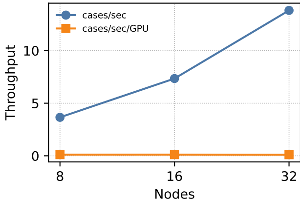
Weak scaling
