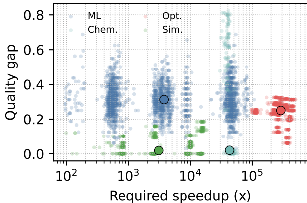
Threshold-quality landscape
