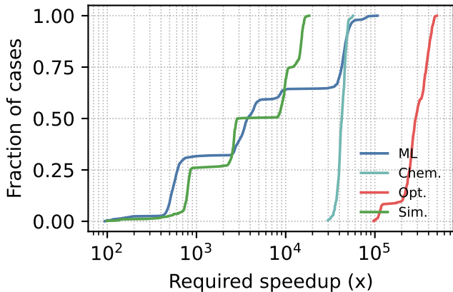
Threshold CDF
