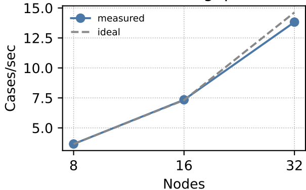
Total throughput
