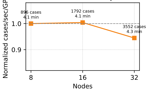
Per-GPU stability
