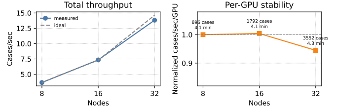
Fig. 6: Weak scaling of the large-profile application suite. Total throughput grows nearly linearly from 8 to 32 nodes while normalized per-GPU throughput remains close to the 8-node reference.
