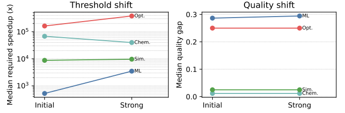
Fig. 5: Native baseline stress test. The slope view shows how each workload moves when the native path is strengthened, instead of hiding the shift inside grouped bars. Strengthening the native side makes the ML threshold 6.6× larger and the optimization threshold 2.3× larger than the initial native-baseline sweep.
