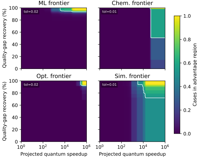
Fig. 8: Advantage frontier over projected quantum speedup and quality-gap recovery. Color shows the fraction of measured cases in each family that would enter the advantage region under that hypothetical hardware and algorithmic improvement. The contour marks the 50% frontier when it appears.
