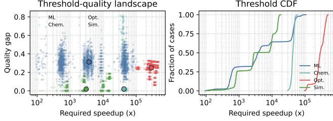
Fig. 4: Large practical-suite landscape over 3,552 cases. The left panel keeps both axes that matter for advantage: required speedup and quality gap. The right panel shows the full threshold distribution rather than only one bar per workload.
