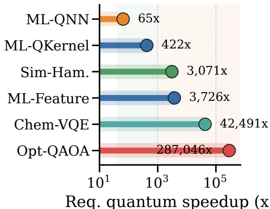
Fig. 1: Application-level threshold examples. The key comparison is not simulator versus simulator. The key comparison is native application execution versus quantum-circuit application execution and projected quantum hardware execution. ML is split into controlled QNN/VQC, controlled QKernel, and practical feature-circuit cases; Sim-Ham. denotes Hamiltonian simulation.
