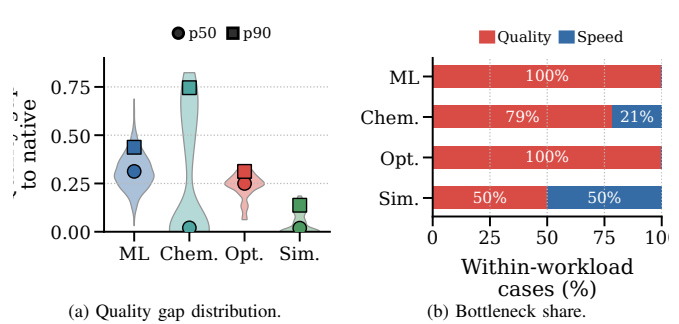
Fig. 9: Quality bottlenecks across the practical suite. Subfigure (a) shows the quality-gap distribution to native, with markers for median and 90th percentile. Subfigure (b) reports within-workload case fractions: cases in a bottleneck class divided by total cases in that workload. A case is quality-limited when its quality gap exceeds the workload tolerance; otherwise, the cases shown here are speed-limited when runtime remains the primary blocker.
