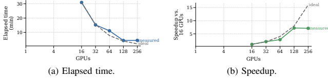
Fig. 12: Strong scaling of the fixed 3,552-case application suite. The run reduces time-to-solution from 30 minutes 55 seconds on 16 GPUs to about 4 minutes 20 seconds on 128–256 GPUs, where task granularity and case imbalance become the limit.
