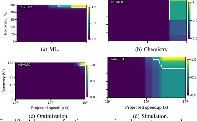
Fig. 13: Advantage frontier over projected quantum speedup and quality-gap recovery. Color shows the fraction of measured cases in each family that would enter the advantage region under that hypothetical hardware and algorithmic improvement. The contour marks the 50% frontier when it appears.
