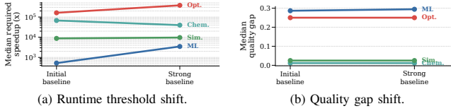
Fig. 9: Native baseline stress test. The slope view shows how each workload moves when the native path is strengthened, instead of hiding the shift inside grouped bars. Strengthening the native side makes the ML threshold 6.6\times larger and the optimization threshold 2.3\times larger than the initial native-baseline sweep.
