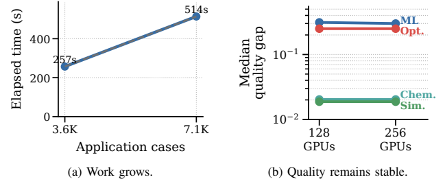
Fig. 10: Larger-workload gate on 256 GPUs. The 256-GPU run completes 7,104 cases in 514 seconds with empty stderr logs. The larger run preserves the workload-level quality interpretation, so the extra cases increase evidence coverage rather than changing the advantage conclusion.
