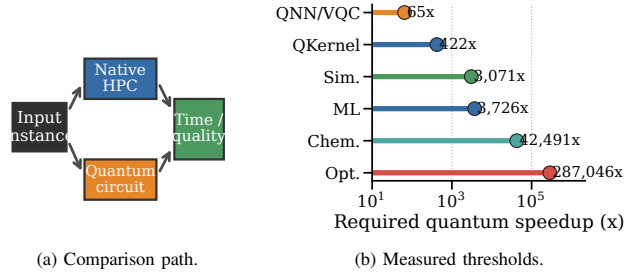
Fig. 1: Application-level comparison target. The key comparison is not simulator versus simulator. The key comparison is native application execution versus quantum-circuit application execution and projected quantum hardware execution.
