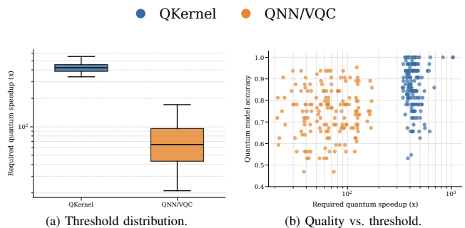
Fig. 6: Expanded digits results over 160 cases. The quantum-kernel path often reaches useful accuracy but needs hundreds of times faster execution, while QNN/VQC has a lower threshold but usually lower quality.
