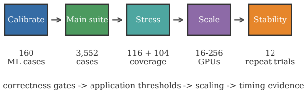
Fig. 5: Completed leadership-system evidence campaign. The figure separates correctness, application coverage, scaling, and timing evidence instead of compressing the evaluation plan into a table.
