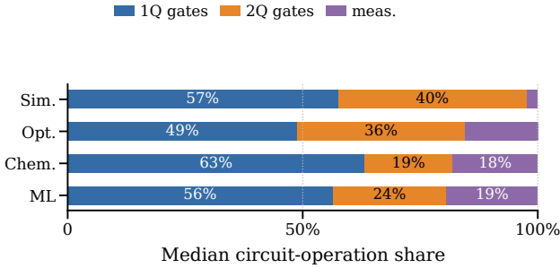
Fig. 8: Circuit-operation pressure by workload. The measured circuit path spends work differently across families: ML is dominated by feature-map evaluations, optimization by repeated QAOA grids, chemistry by VQE term evaluation, and simulation by fewer but state-evolution-heavy circuits.
