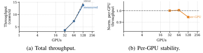
Fig. 11: Weak scaling of the comparable large-profile application suite. Total throughput grows nearly linearly from 32 to 128 GPUs while normalized per-GPU throughput remains close to the 32-GPU reference.
