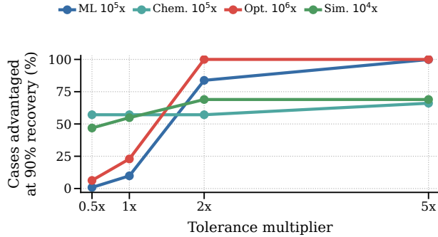
Fig. 13: Tolerance sensitivity of the advantage frontier. The same measured cases can be reinterpreted under stricter or looser quality budgets; this changes quality-limited ML and optimization much more than speed-bound chemistry.
