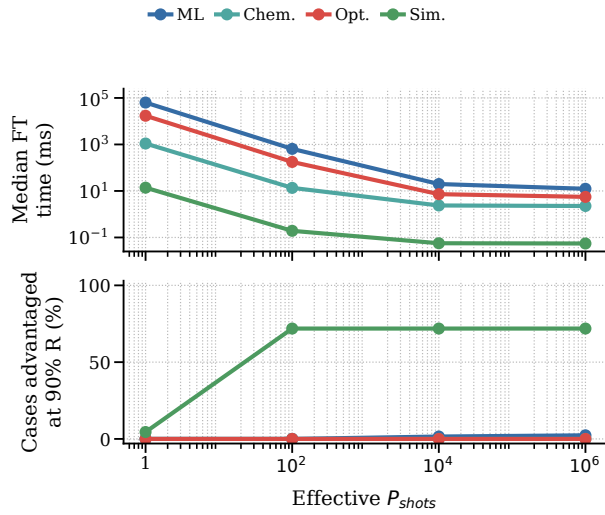
Fig. 14: Concrete FT-stack and shot-parallelism sensitivity. The same measured metadata is evaluated under a stylized surface-code stack. Runtime falls as P_{\text{shots}} increases, but the serial decoder/control floor and quality gate leave chemistry, ML, and optimization constrained even when logical gate work is highly parallel.
