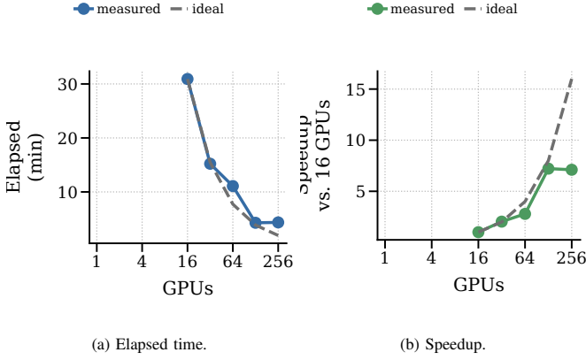
Fig. 11: Strong scaling of the fixed 3,552-case application suite. The run reduces time-to-solution from 30 minutes 55 seconds on 16 GPUs to about 4 minutes 20 seconds on 128–256 GPUs, where task granularity and case imbalance become the limit.
