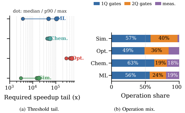
Fig. 6: Tail and circuit pressure by workload. The left plot shows median, 90th percentile, and maximum threshold pressure; the right plot separates one-qubit, two-qubit, and measurement pressure after the fixed simulation floor is removed.
