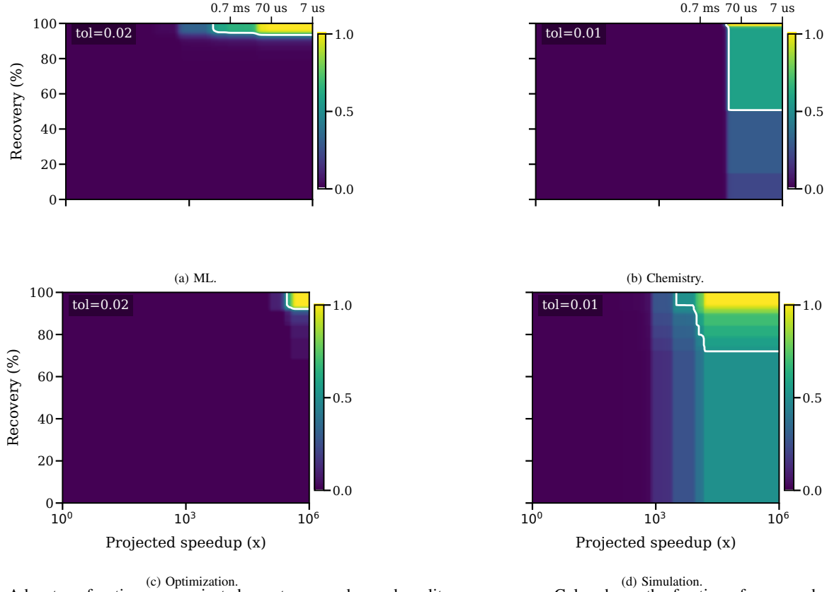
Fig. 12: Advantage frontier over projected quantum speedup and quality-gap recovery. Color shows the fraction of measured cases in each family that would enter the advantage region under that hypothetical hardware and algorithmic improvement. The top-row secondary axis maps speedup to effective quantum execution time using the measured seven-second circuit path; the contour marks the 50% frontier when it appears.
