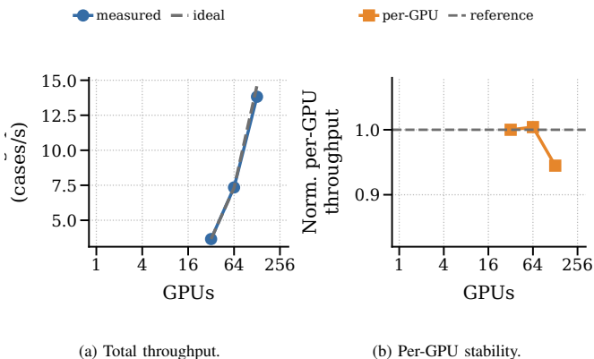
Fig. 10: Weak scaling of the comparable large-profile application suite. Total throughput grows nearly linearly from 32 to 128 GPUs while normalized per-GPU throughput remains close to the 32-GPU reference.
