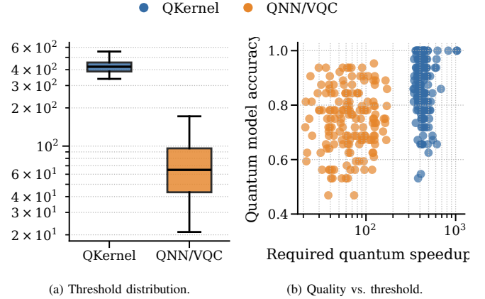
Fig. 4: Expanded digits results over 160 cases. The quantum-kernel path often reaches useful accuracy but needs hundreds of times faster execution, while QNN/VQC has a lower threshold but usually lower quality.
