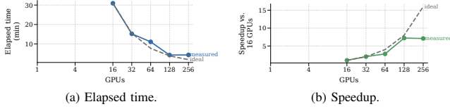
Fig. 13: Strong scaling of the fixed 3,552-case application suite. The run reduces time-to-solution from 30 minutes 55 seconds on 16 GPUs to about 4 minutes 20 seconds on 128–256 GPUs, where task granularity and case imbalance become the limit.
