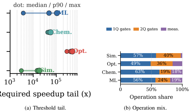
Fig. 8: Tail and circuit pressure by workload. The left plot shows median, 90th percentile, and maximum threshold pressure; the right plot separates one-qubit, two-qubit, and measurement pressure after the fixed simulation floor is removed.
