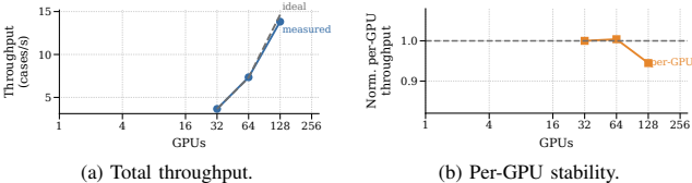
Fig. 12: Weak scaling of the comparable large-profile application suite. Total throughput grows nearly linearly from 32 to 128 GPUs while normalized per-GPU throughput remains close to the 32-GPU reference.
