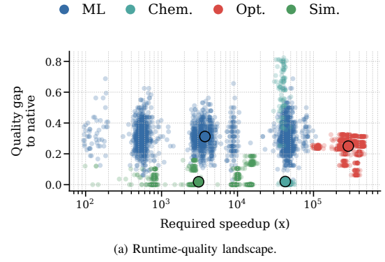
Fig. 7: Large practical-suite landscape over 3,552 cases. The plot keeps both axes that matter for advantage: required speedup and quality gap. A workload is not close to advantage unless it moves left in runtime and down in quality gap.
