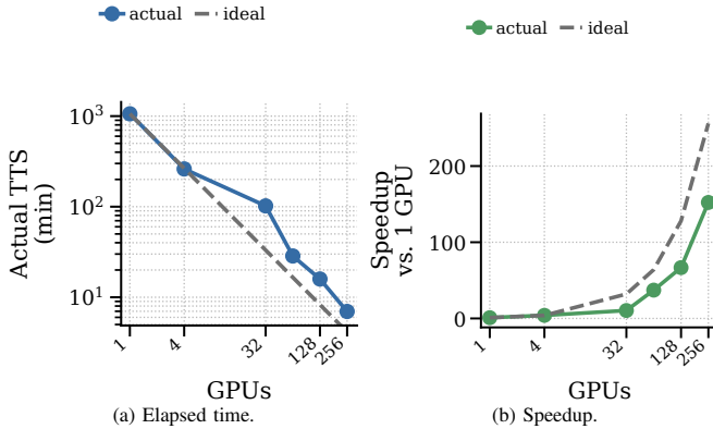
Fig. 6: Strong scaling of the fixed 7,104-case application suite. Both subfigures show the actual normalized fixed-work curve against ideal case-level scaling. The 1–32 GPU points are normalized from completed lower-end runs, while the 64–256 GPU points are direct fixed-suite regular-queue runs. The measured full run reduces time-to-solution from 28 minutes 33 seconds on 64 GPUs to 6 minutes 58 seconds on 256 GPUs.
