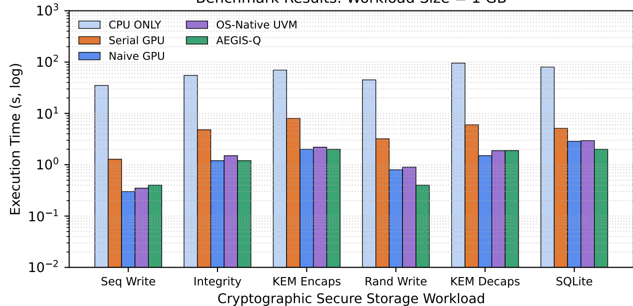
Benchmark Results: Workload Size = 1 GB
