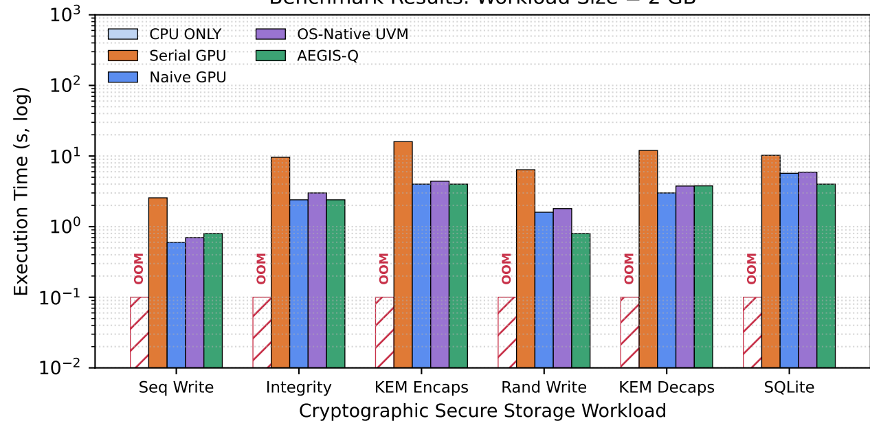
Benchmark Results: Workload Size = 2 GB
