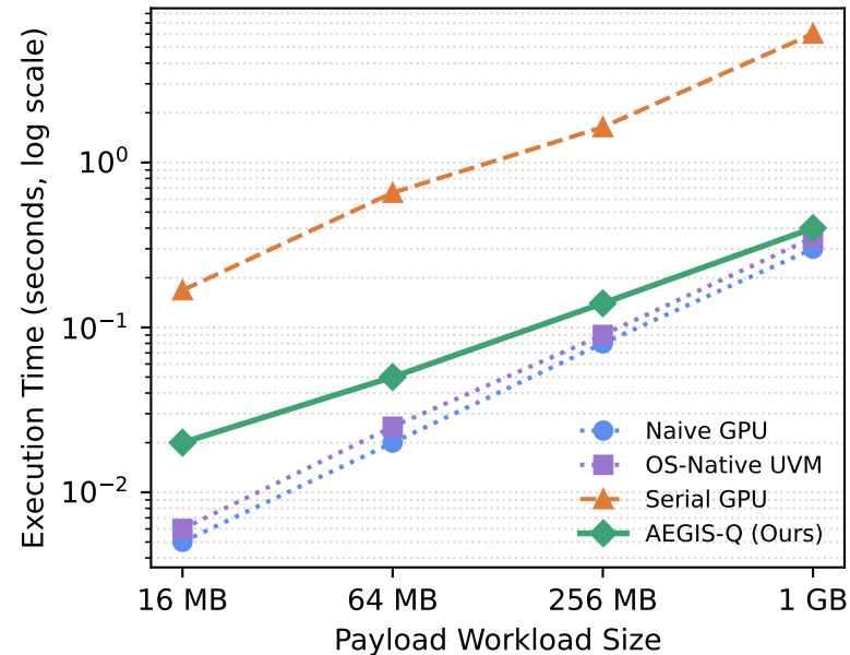
PQC Staging Performance
