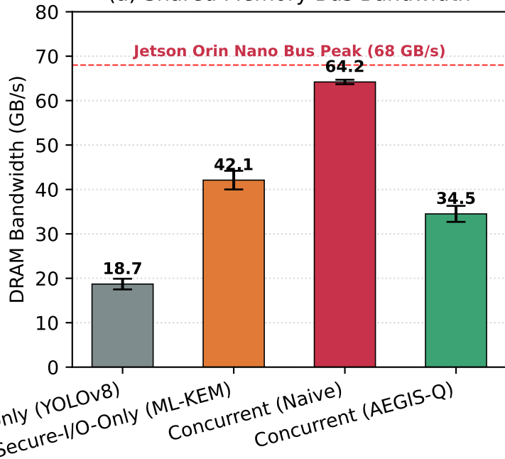
(a) Shared Memory Bus Bandwidth
