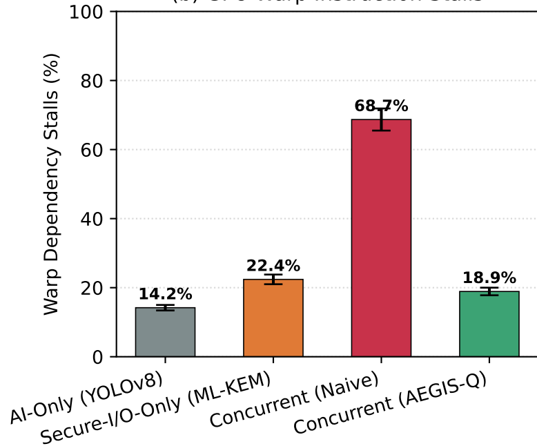
(b) GPU Warp Instruction Stalls
