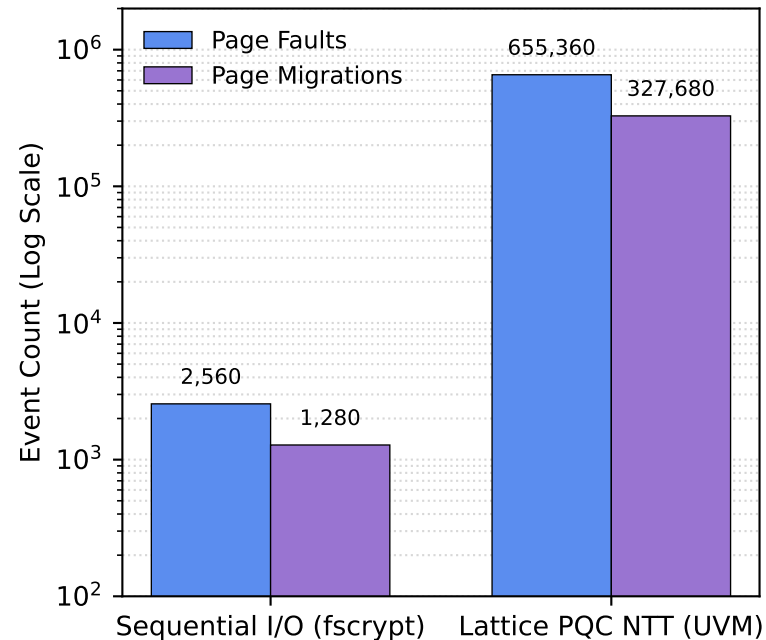
(a) Kernel Memory Event Overheads
