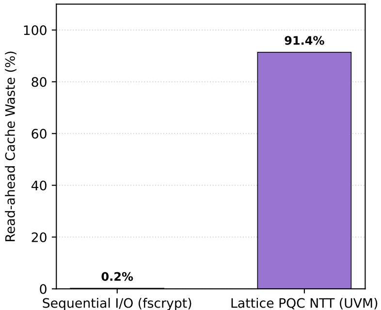
(b) OS Page Cache Read-ahead Waste
